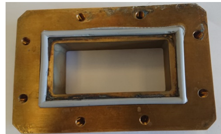
Figure 5: Flange with arcing burns and pinched gasket.
