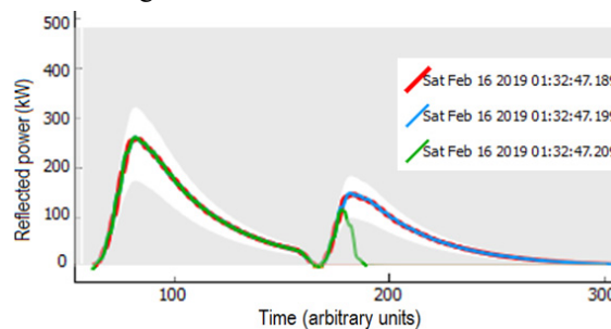
Figure 2: Breakdown event in reflected power trace. The red and blue traces are the normal pulses before the green trace which has a breakdown. Anything outside the white region for a chosen number of points in time is classed as a breakdown.
