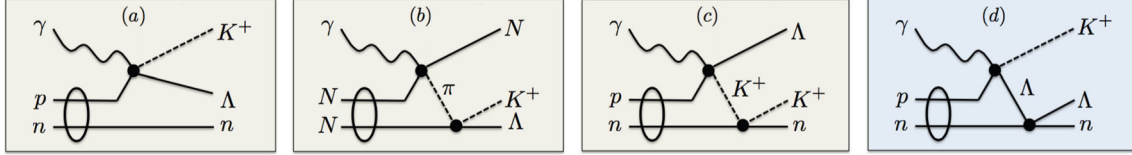
Fig. 6 Four main mechanisms that contribute to the reaction \gamma d \rightarrow K^+ \Lambda n according to theoretical models [16,17]: a quasi-free \Lambda photoproduction on the proton; b pion mediated production; c K^+ rescattering on spectator neutron; d \Lambda rescattering on spectator neutron (Colour figure online)
