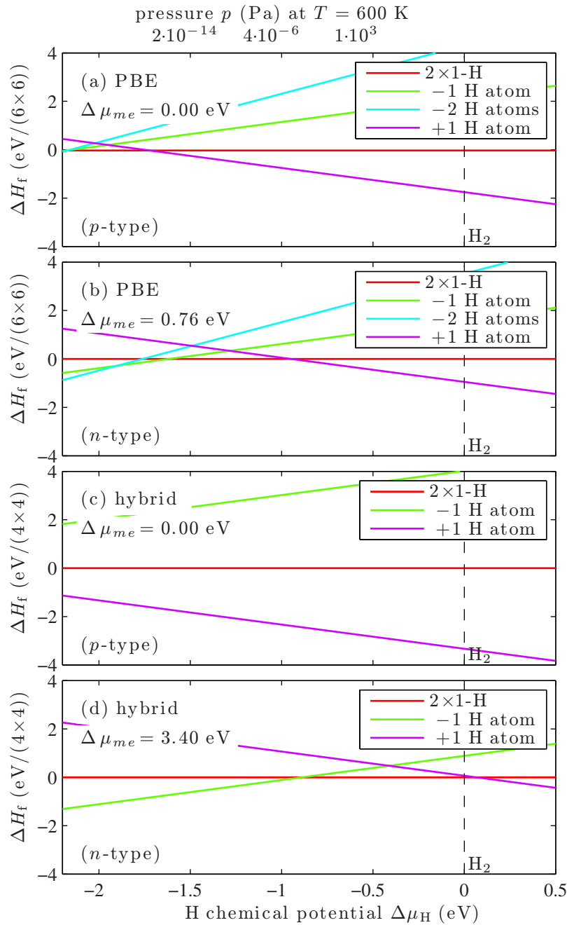
Figure 4. The four surface structures considered are plotted as a function of the H chemical potential \Delta \mu_H for (a) PBE functional and p-type conditions, (b) PBE functional and n-type conditions, (c) hybrid functional and p-type conditions and (d) hybrid functional and n-type conditions.
