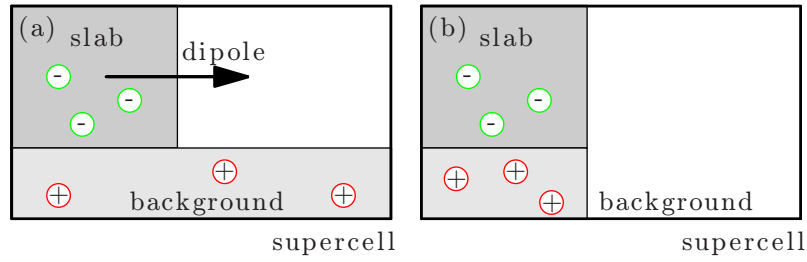
Figure 2. (a) The introduction of negative charge into a periodical supercell requires a positive compensating background. The uniform background leads to a dipole, which diverges upon increasing the amount of vacuum in the supercell. (b) Confining the compensating charge to the extension of the slab in the surface supercell prevents the build up of an undesired dipole.
