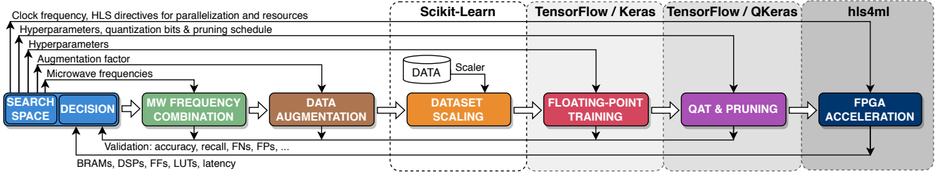
Fig. 1: The proposed enhanced ML flow.
