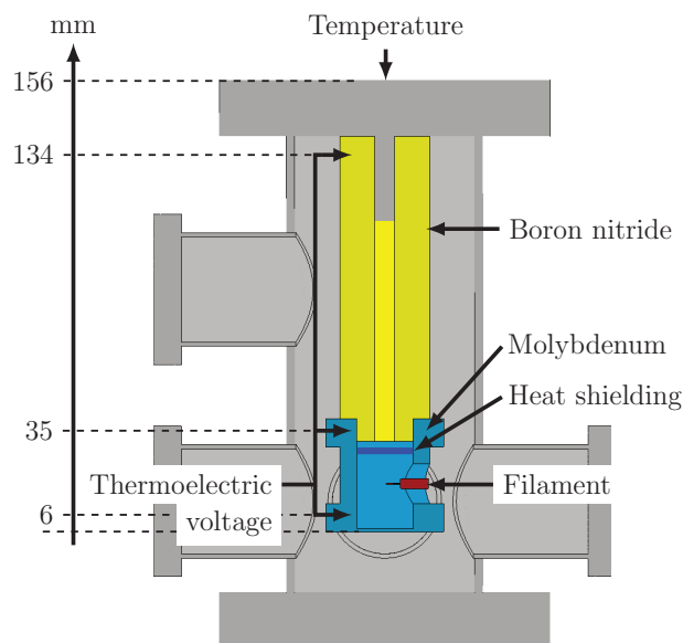
Figure 3: Sketch of the Heating experiment. The Mo body is irradiated with a halogen filament from inside and shielded from the BN rod.
