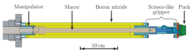
Figure 2: CAD model of the gripper. A dual-axis manipulator is used. The yellow parts are insulating materials (BN respectively Macor).
