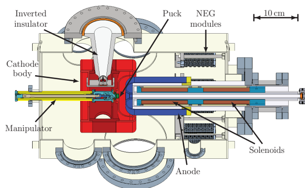
Figure 1: CAD model of MIST. The cathode (red) to anode (blue) distance is 22 mm. The photocathode is mounted in a puck (green). The puck-transfer-manipulator remains all the time during operation in the source.
