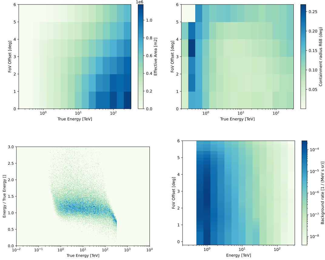
Figure 1: Top-left: effective area in terms of true energy and offset from the center of the FoV. Top-right: Containment radius at 68% of the PSF as a function of true energy and offset. Bottom-left: dispersion matrix (stacked over the whole offsets). Bottom-right: background rate as a function of energy and offset.
