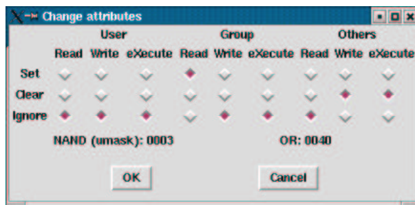
Figure 6: Attributes changing
