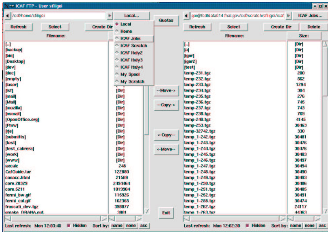
Figure 5: ICAF GUI
