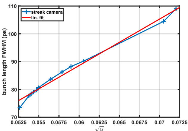
Figure 4: FWHM bunch length measured by streak camera (blue) versus square root of the momentum compaction factor \alpha_c and linear fit to the data (red).
