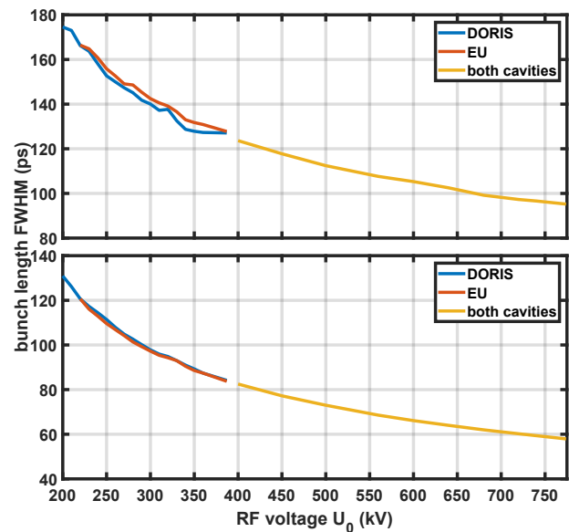
Figure 3: FWHM bunch length measured by a streak camera (top) and deduced from the synchrotron frequency (bottom) as function of the RF voltage U_0 . Data are shown for operating only the DORIS cavity (blue), only the EU cavity (red) and both (yellow).
