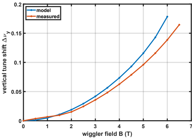
Figure 1: Vertical tune shift \Delta\nu_y as function of the wiggler field B without any compensation. The tune shift given by the optics model is shown in blue, the measured tune shift in red.
