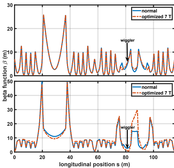
Figure 2: Horizontal (top) and vertical (bottom) beta function \beta as function of the longitudinal position s without wiggler (blue) and optimized at 7 T (red).
