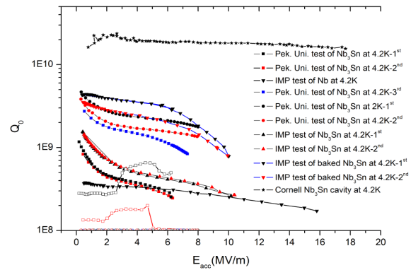
Figure 9: Vertical test results of the Nb_3Sn cavity coated at Peking University and IMP.
