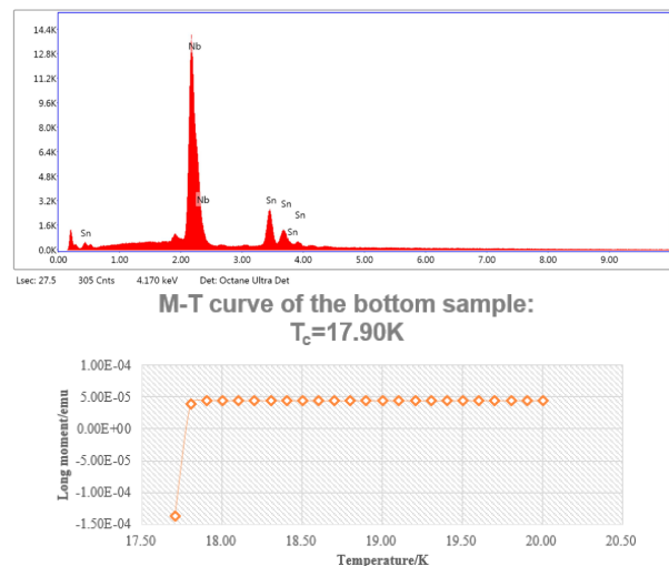
Figure 2: EDS spectrum of the first batch Nb 3 Sn samples indicates composition 24.49 At. % Sn (top); T_c of the first batch Nb 3 Sn samples reached ~17.9K
