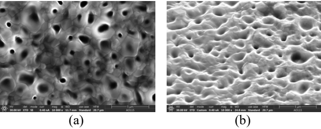
Figure 12: SEM pictures obviously showed many voids on the surfaces of the 2 nd and 3 rd batch samples.
