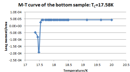
Figure 11: T_c of the Nb_3Sn samples coated with the 2 nd and 3 rd cavity is about 17.6K.
