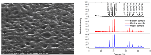
Figure 3: SEM images of the first batch samples tilted at 55° to show three-dimensional features (left); XRD results showed no undesired low-T c phases were detected (right).
