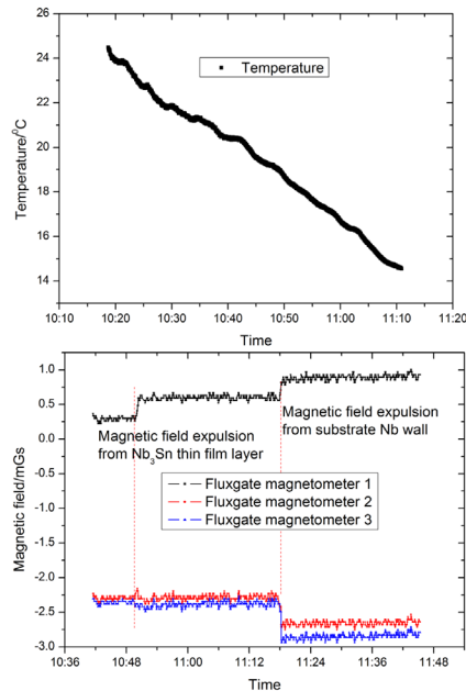
Figure 8: (Top) A slow cooldown of \sim 5.23 min/K was achieved at Peking University; (Down) Magnetic field expulsion was observed during the cooldown at Peking University.
