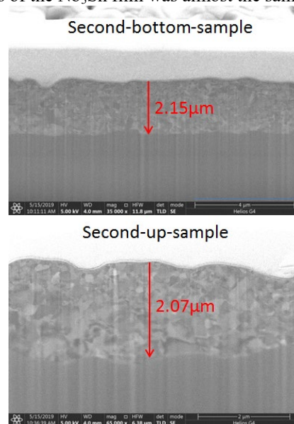
Figure 7: With the modified coating process that kept the Sn source and the cavity at 1200°C for 3 hours, the thickness of the bottom sample and the upper sample is almost the same.
