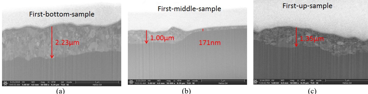
Figure 5: Profiles of layers made visible by ion beam of the bottom sample (a), the central sample (b) and the upper sample (c).
