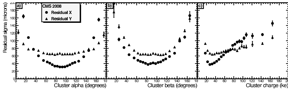
Figure 2: Pixel hit residuals as function of the transverse and longitudinal impact angles and cluster charge in kiloelectrons. The full circles correspond to the transverse coordinate and the full triangles to the longitudinal coordinate. Tracks have a momentum larger than 10 GeV/c. Impact angles of 90^\circ correspond to normally incident tracks.
