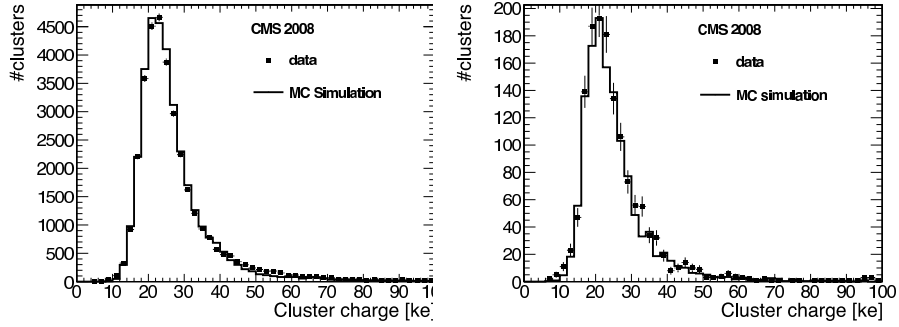
Figure 1: Charge distribution in kiloelectrons (ke) for clusters larger than one pixel measured with the barrel and endcap pixel detector in the first and second plot respectively. The data points show the measurement with cosmic rays and the solid line the simulation.
