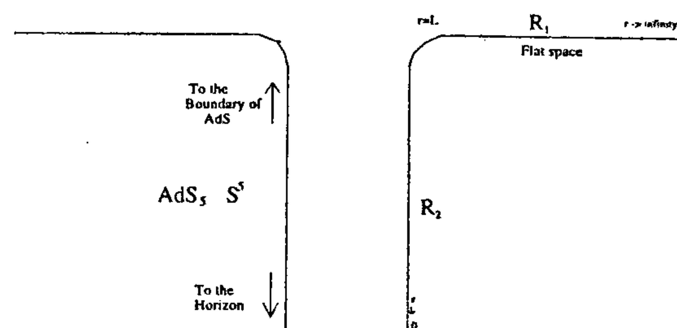
Figure 5. A crude depiction of the 3-brane geometry. Each point on either of the two lines represents a 9 dimensional subspace at constant r , the product of an S^5 (surrounding the 3-branes in 6 dimensional transverse space), and an R^4 (or T^3 \times R for finite branes) the spacetime along the 3-branes. Arc length along the curves in the diagram measures proper distance along the radial direction. r decreases from \infty to zero as one runs down the curve and r = 0 is infinitely far down the tube. The distance of any point from the axis of the diagram represents the radius of the S^5 at that point. For finite branes wrapped on a torus T^3 the size of the torus stays constant along the horizontal line, but shrinks on descending the tube, tending to zero at the bottom.
