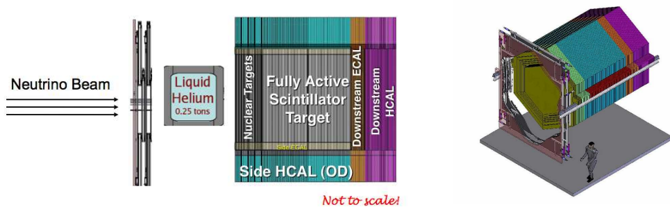
Fig. 2. Left: Side view of the MINER \nu A experiment. Right: Three dimensional view of the MINER \nu A detector.
