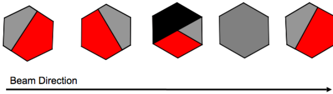
Fig. 3. Geometry of the nuclear targets in MINER \nu A. The targets are stacked in the detector in the order shown, from left to right. Four scintillator modules are placed between each target. Deep gray (red): Fe, gray: Pb, black: C.
