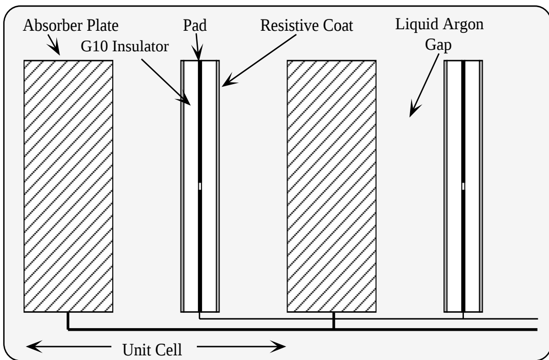
Figure 3.8: Unit cell in the DØ calorimeter.
