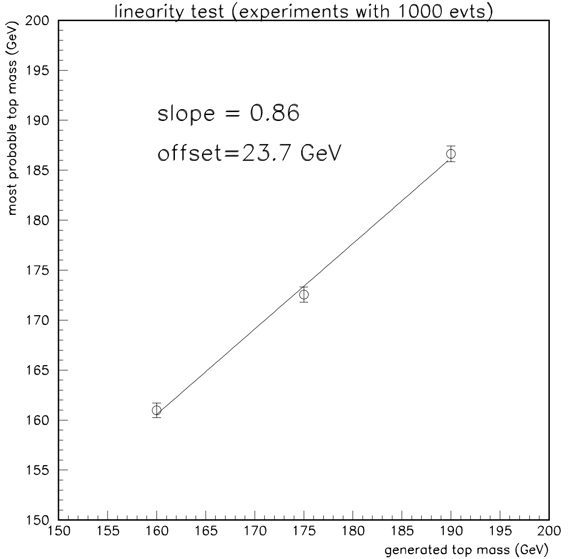
Figure 7.1: Most probable values of the mass of the top quark obtained for simulated experiments of 1000 events, generated with a m_t=160 , 175 and 190 GeV. The standard DØ jet energy corrections were used in this study.
