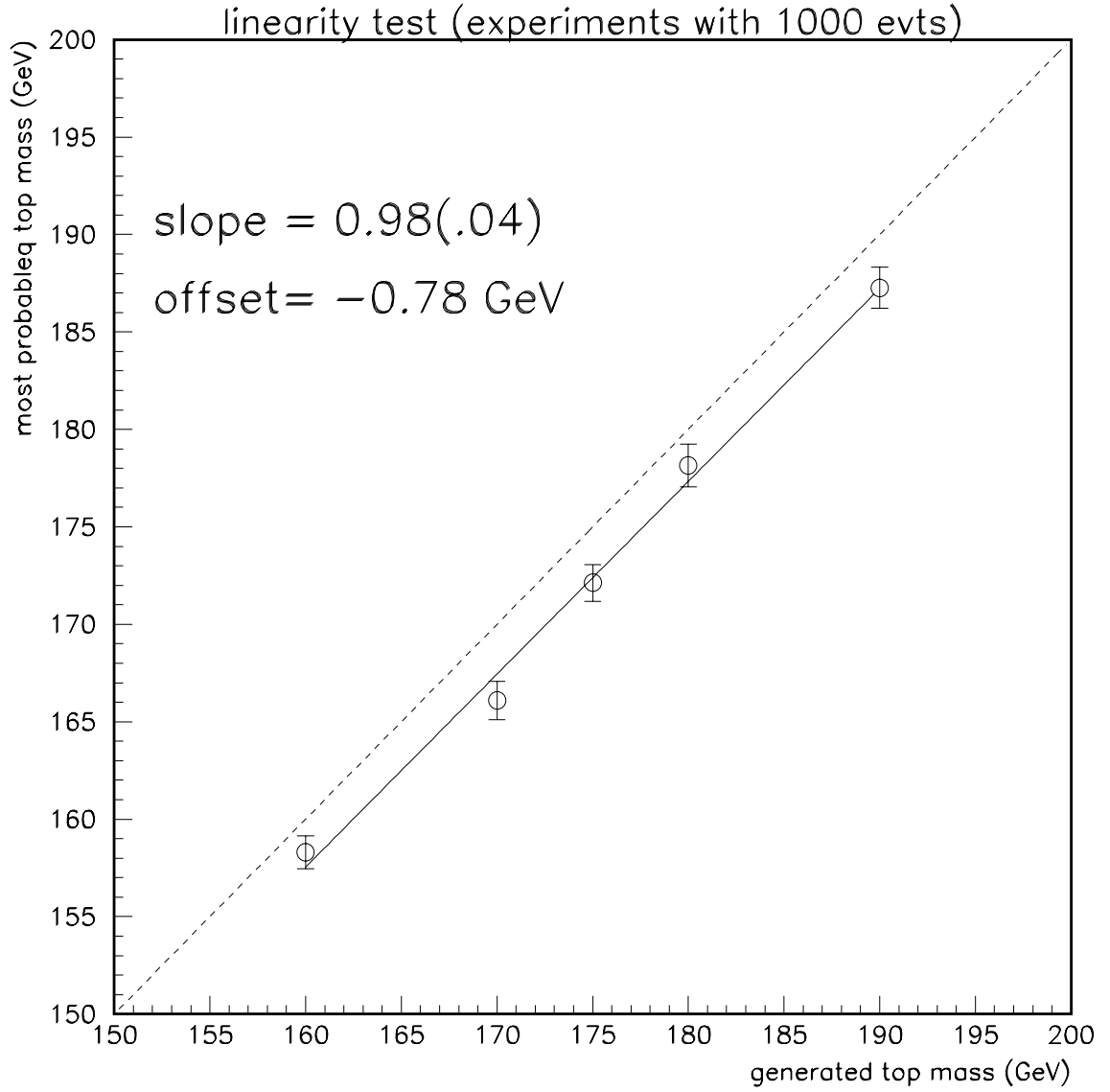
Figure 7.2: Most probable values of the mass of the top quark obtained for simulated experiments of 1000 events, generated with a m_t=160, 170, 175, 180 and 190 GeV. The complete transfer functions were used in this study.
