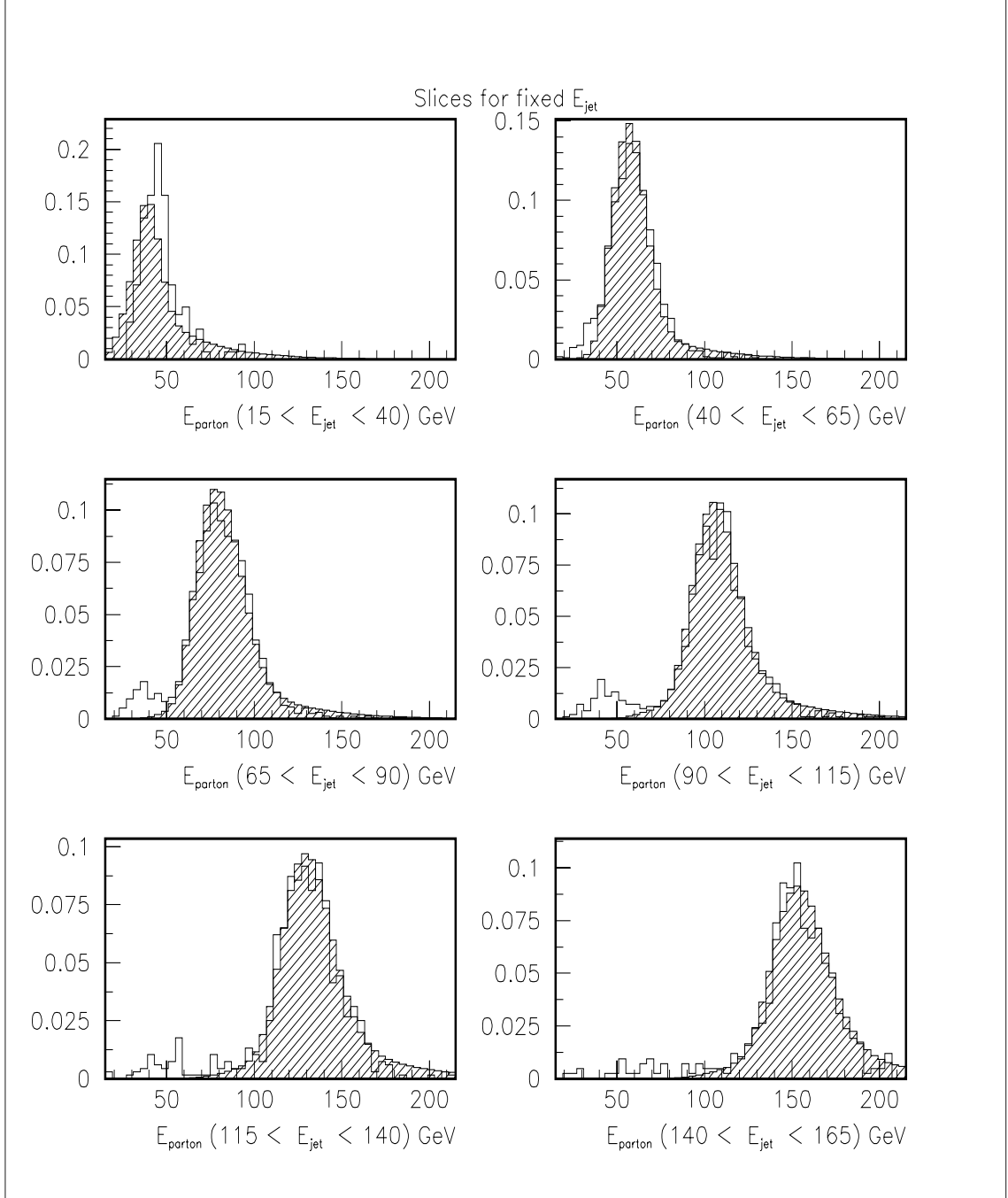
Figure 5.6: Slices in E_{jet} , same plots as in Figure 5.4, but now for jets in the region 1.3 < |\eta| < 2.0 .
