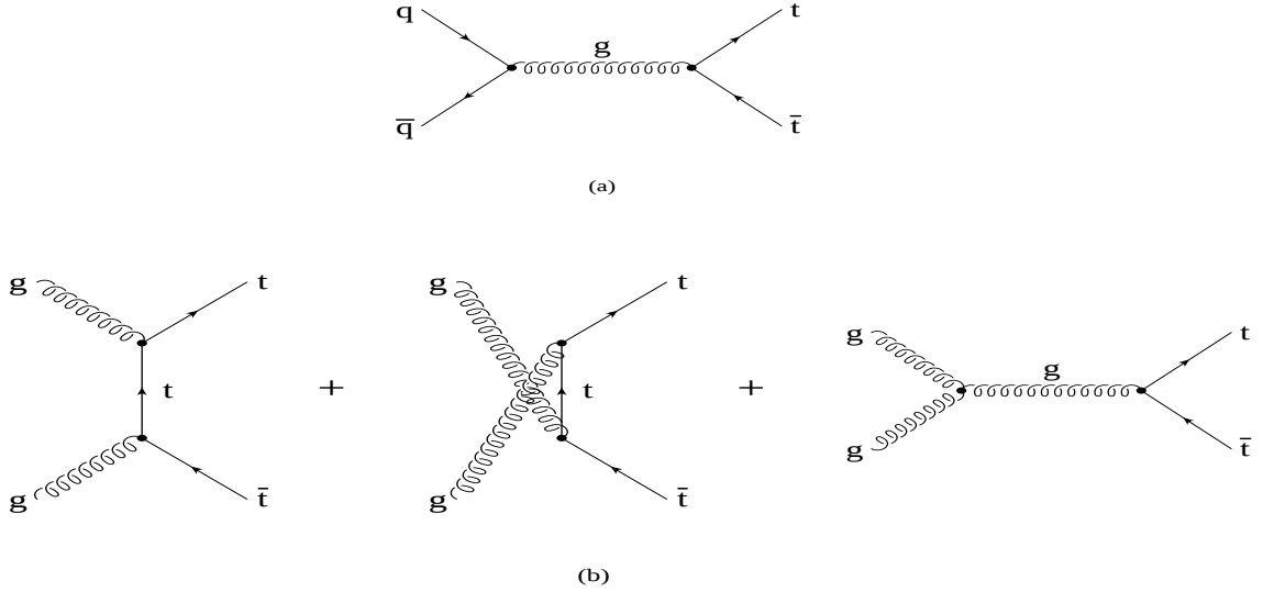
Figure 2.2: Leading order diagrams for t\bar{t} production.
