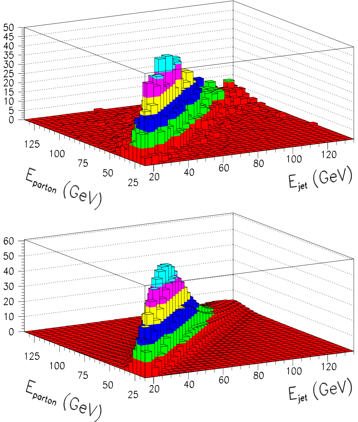
Figure 5.2: Top: lego plot of E_{parton} vs E_{jet} for a sample of jets associated with partons in t\bar{t} Monte Carlo events, using full DØ detector simulation (CAFIX corrections included). Bottom: lego plot of E_{parton} vs E_{jet} , where E_{parton} is predicted using n(E_{parton}) and the transfer function described in Eq.(5.2). The jets are in the region of 0.2 < |\eta| < 0.6 .
