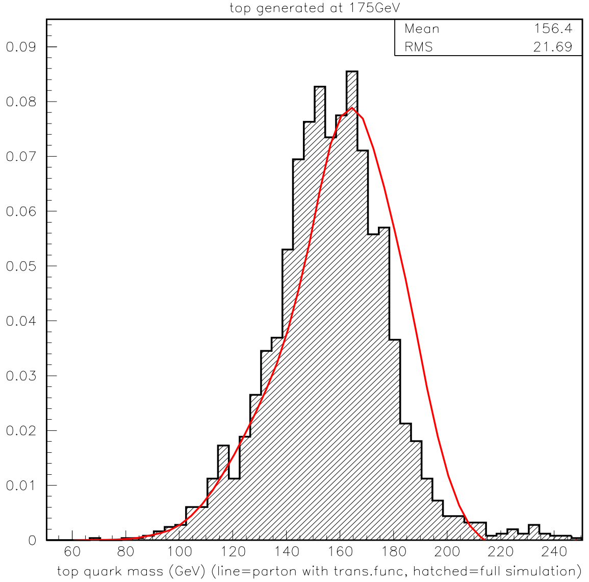
Figure 5.8: Same as Figure 5.7, but now m_t=175 GeV.
