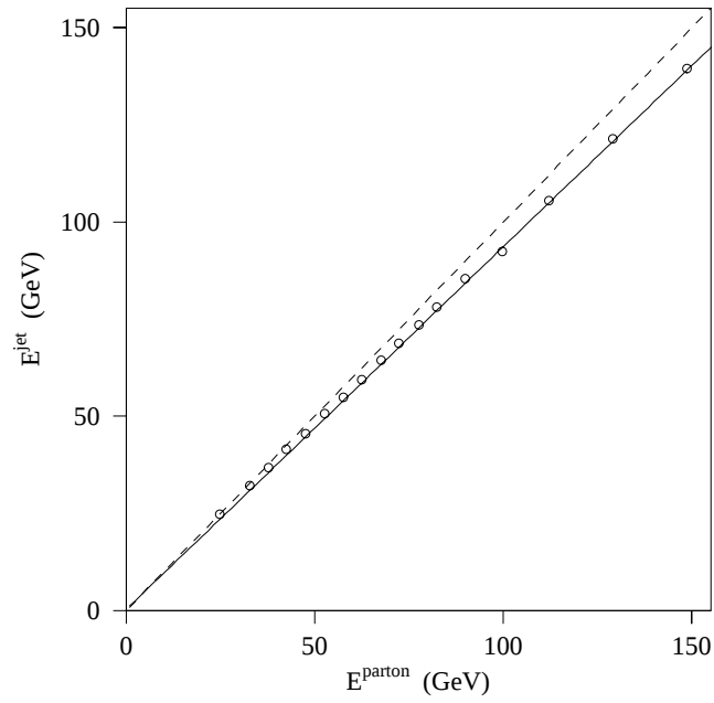
Figure 4.1: Effect of the out-of-cone radiation. The reconstructed jets have on average less energy than the original parton, this is the motivation for the out-of-cone corrections, which are based on the comparison of parton energies and energies of reconstructed jets in t\bar{t} events (circles). The correction attempts to provide a 1:1 correspondence ( given by the dashed line).
