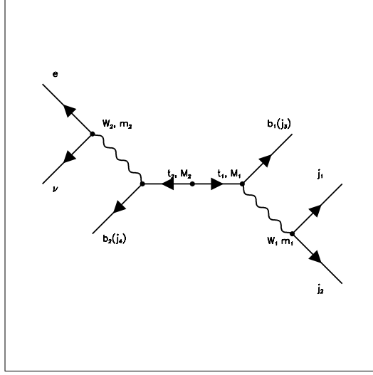
Figure B.1: Feynman diagram for the single-lepton t\bar{t} event.
