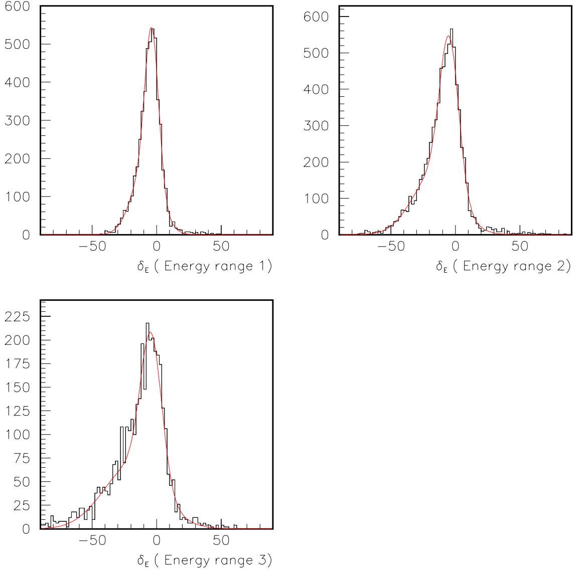
Figure 5.1: Distributions in \delta_E = E_{jet} - E_{parton} for different parton energy ranges ( E range 1: 15 \text{ GeV} < E_{parton} < 60 \text{ GeV} , E range 2: 60 \text{ GeV} < E_{parton} < 100 \text{ GeV} , E range 3: 100 \text{ GeV} < E_{parton} < 140 \text{ GeV} , for jets in t\bar{t} event with 0.2 < |\eta| < 0.6 ). The distributions have an extended tail for \delta_E < 0 , which corresponds to the effect of hadronization and radiation.
