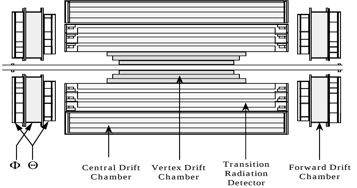
Figure 3.3: Schematic of the DØ central tracker.
