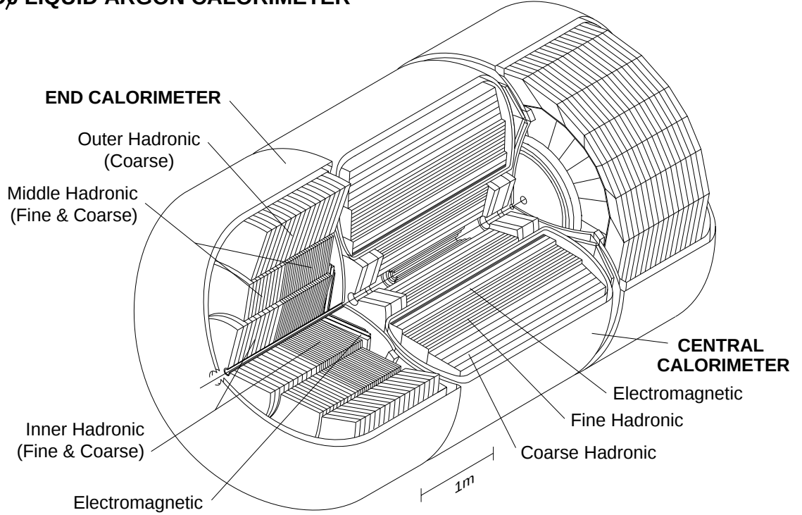
Figure 3.6: Schematic of the DØ calorimeter
