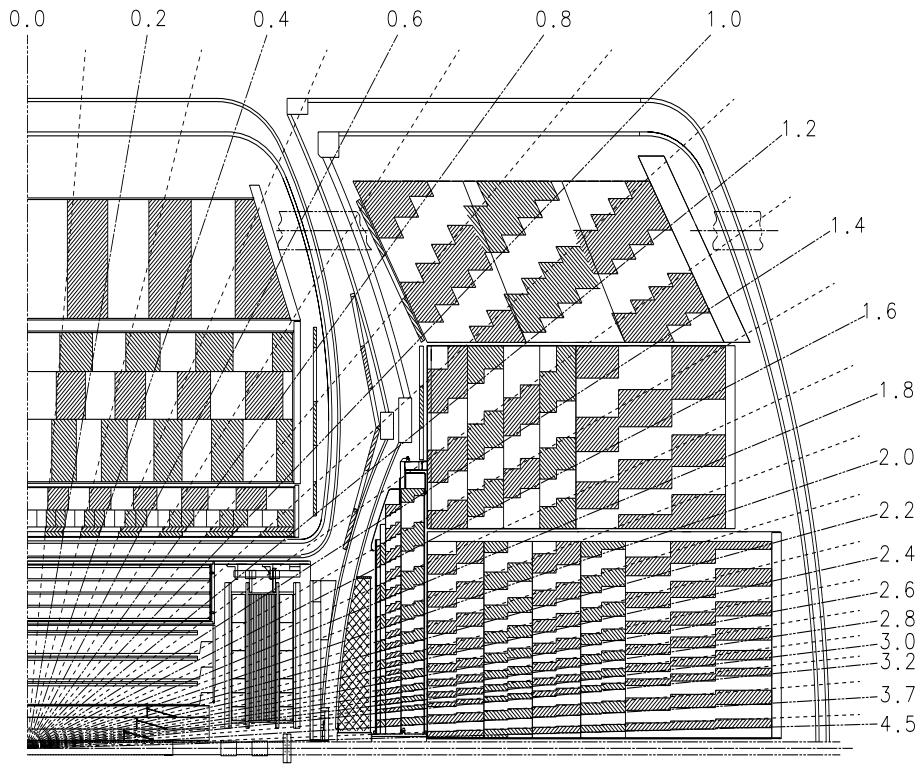
Figure 3.7: Side view of the DØ calorimeters. Rays of fixed \eta relative to the center of the detector are given in the sketch.
