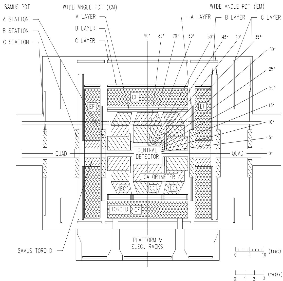
Figure 3.9: Muon Spectrometer in the DØ detector.
