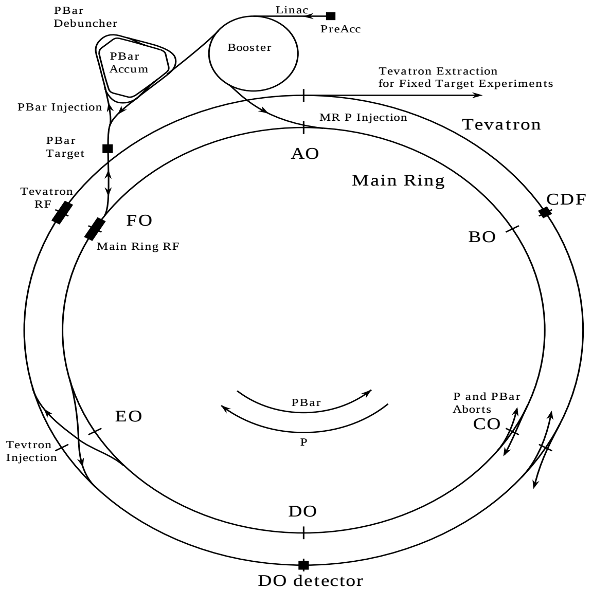
Figure 3.1: Schematic of the accelerator complex
