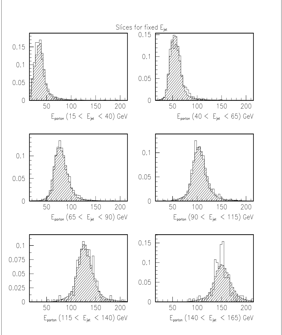
Figure 5.4: Slices of E_{jet} from the plots in Figure 5.2. The filled histogram correspond to predictions using n(E_{parton}) and the transfer function, and the lines correspond to the original MC simulated events.
