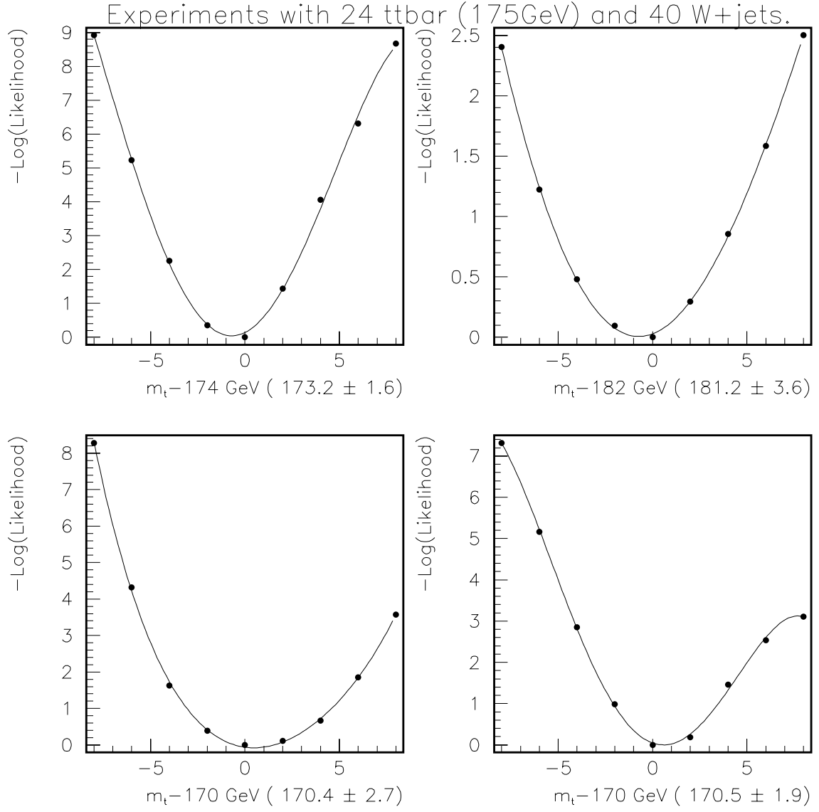
Figure 7.3: -\ln(\text{Likelihood}) for 4 Monte Carlo experiments with 24 signal events and 40 background events, all generated at M_t = 175 \text{ GeV} . The numbers in parentheses indicate the most probable value of the mass of the top quark for each experiment. The x -axis on the plots has been offset to give the minimum always around x = 0 and a constant was subtracted to the likelihood function for convenience.
