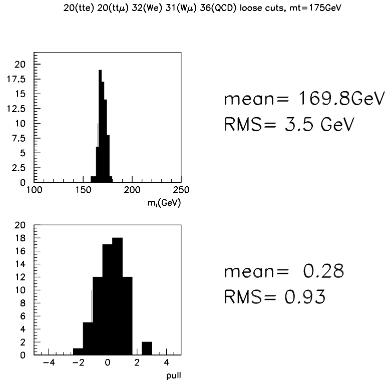
Figure 7.6: Ensemble test with Sample 2. The upper plot shows the results of the most probable mass obtained in different experiments, and the lower plot shows its pull distribution.
