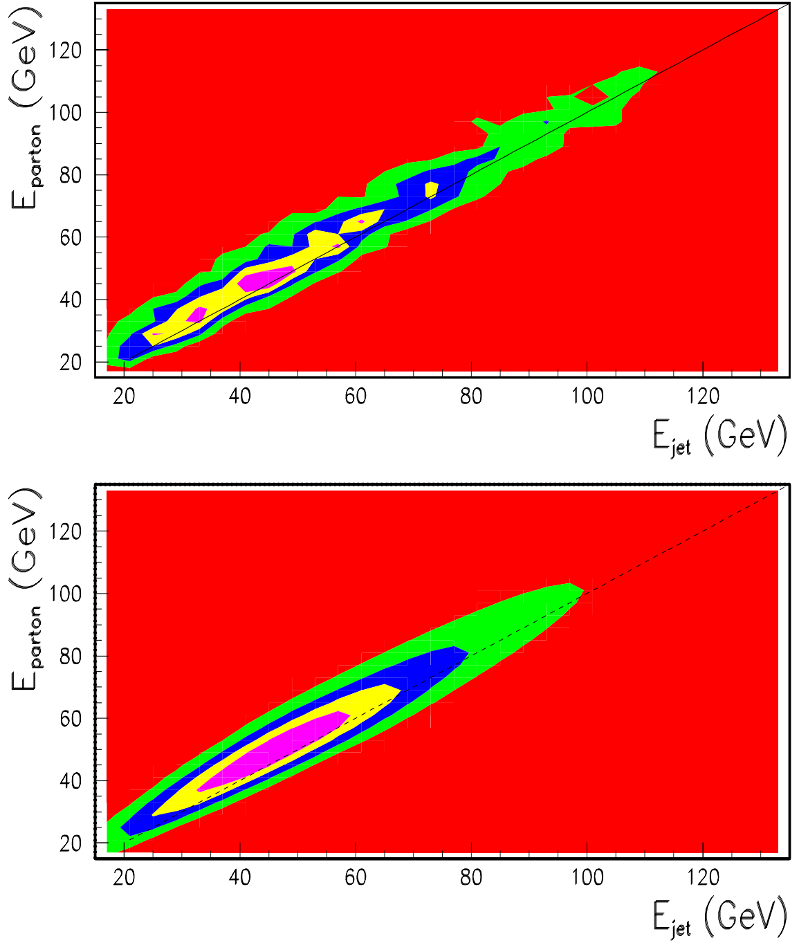
Figure 5.3: Contour plots corresponding to Figure 5.2. The different shadings correspond to different number of events (40, 30, 20, 10 and 5).
