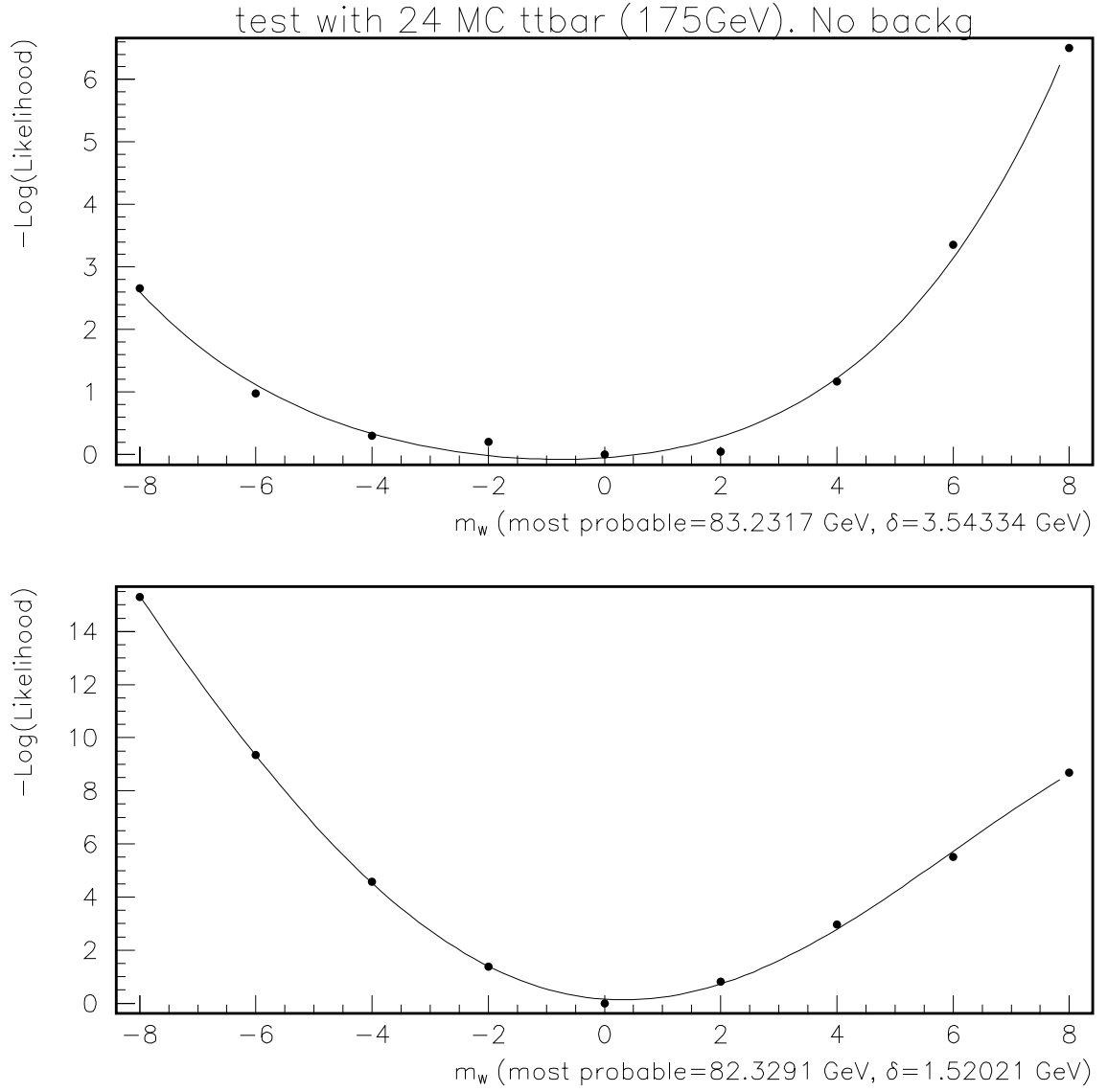
Figure 7.9: Two examples of likelihood as a function of the mass of the W boson in the hadronic channel for a sample of 24 signal t\bar{t} events with no background.
