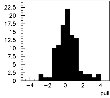
Figure 7.4: Ensemble tests with Sample 1. The upper plot shows the results for the most probable mass extracted in different MC experiments, and lower plot shows the pull distribution in the mass.
