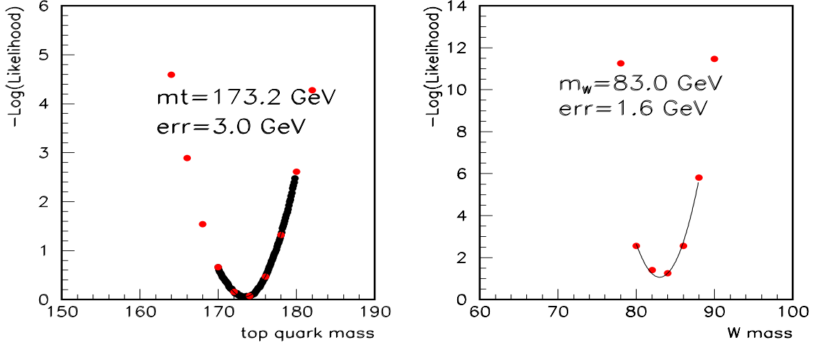
Figure 8.1: Top left(right): Likelihood as a function of m_t(m_W) for 46 e + 4 jets events in the DØ Run I data. Bottom left(right): Likelihood as a function of m_t(m_W) for 46 e+4 jets and 41 muon+4 jets events in DØ Run I data.
