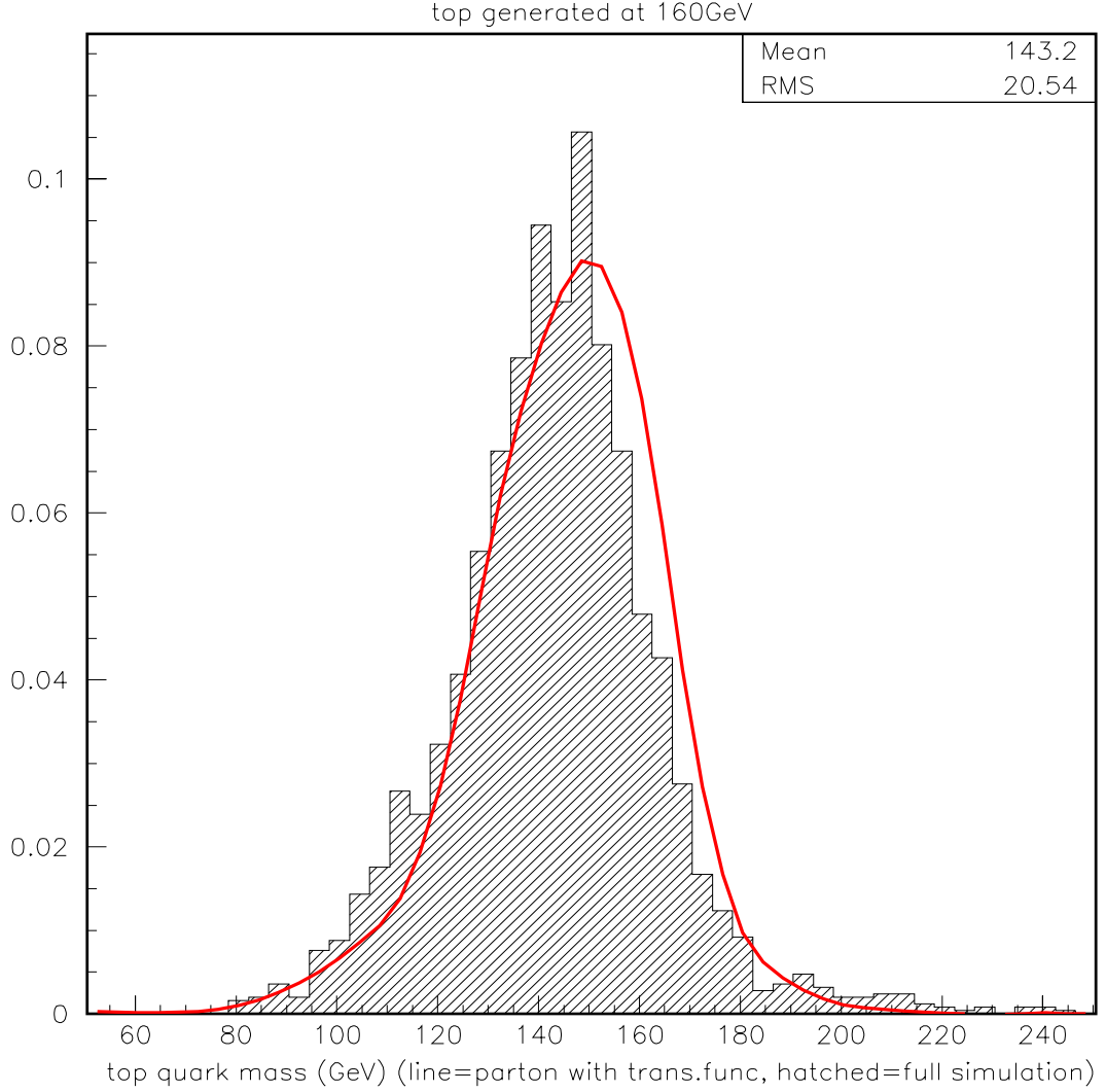
Figure 5.7: Distribution of the invariant mass of three jets with full DØ simulation and CAFIX energy corrections (jets identified in Monte Carlo as coming from the hadronic decay of the top quark) is compared with the prediction from the transfer function. The comparison is done for events simulated with m_t=160 GeV. The mean and RMS values correspond to the hatched histogram.
