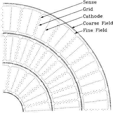
Figure 3.4: The r - \phi view of a quadrant of the Vertex Drift Chamber (VTX).
