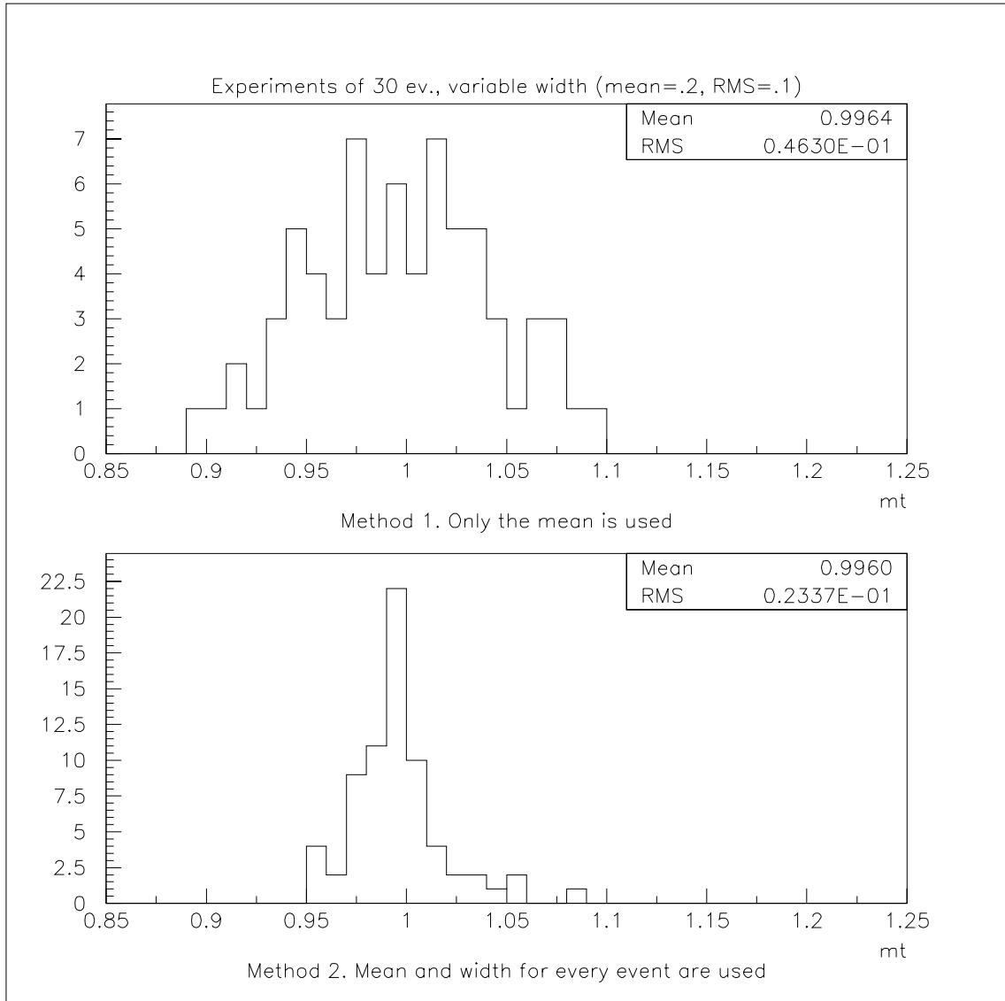
Figure A.2: Histograms of estimators of \langle x \rangle obtained from 80 samples of 30 events using Method I (top) and Method II (bottom). The input events have large differences in uncertainties.
