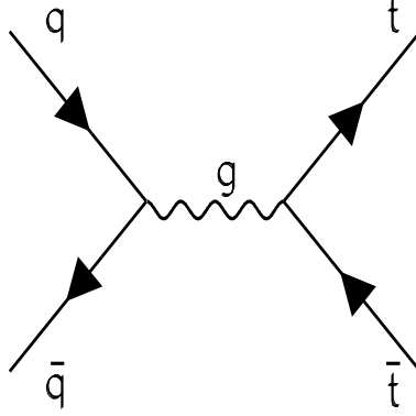
Figure 1.1: Quark and an antiquark can annihilate to produce a gluon, which in turn breaks up into a different quark-antiquark pair, in this case a t\bar{t} pair.
