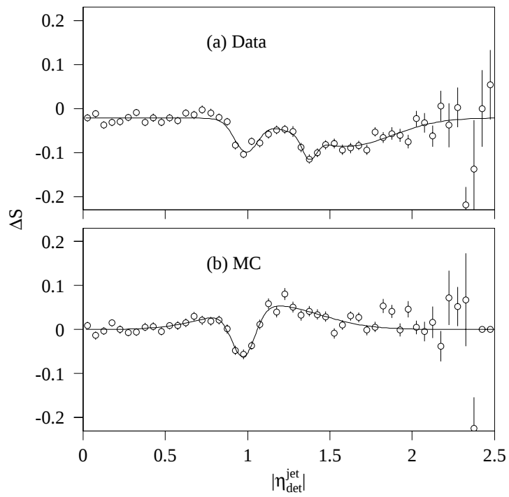
Figure 4.2: Dependence of the deviation in the jet energy scale ( \Delta S ) for \gamma +jets data and t\bar{t} MC events, as a function of |\eta| [45].
