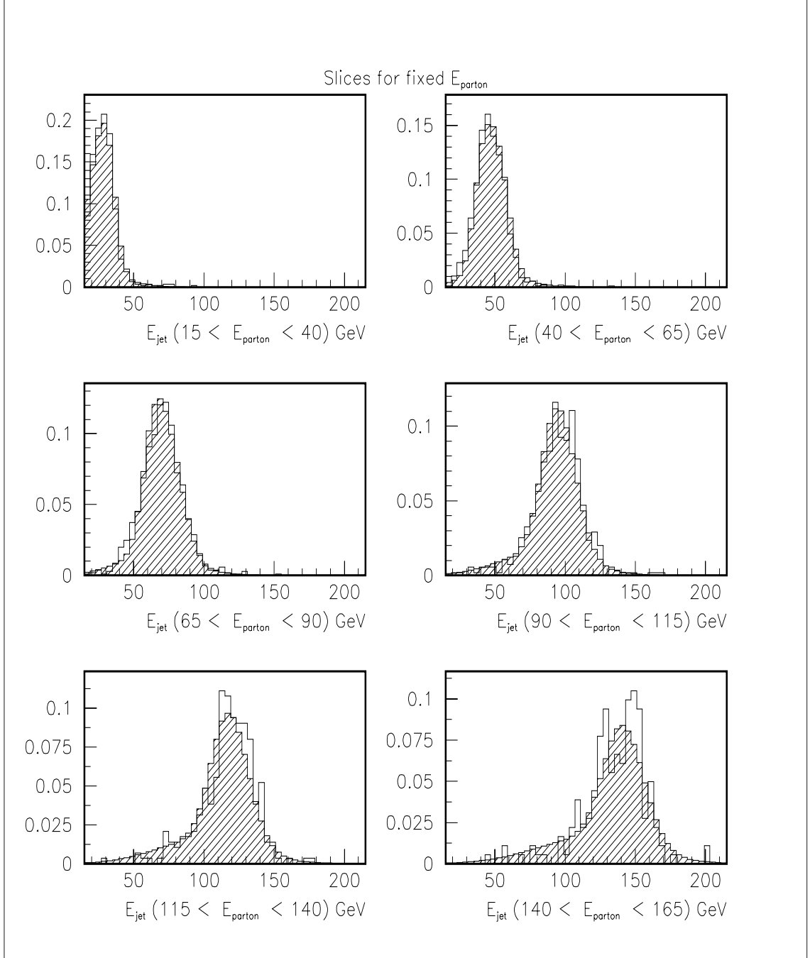
Figure 5.5: Same as Figure 5.4, but now the slices in E_{\text{parton}}
