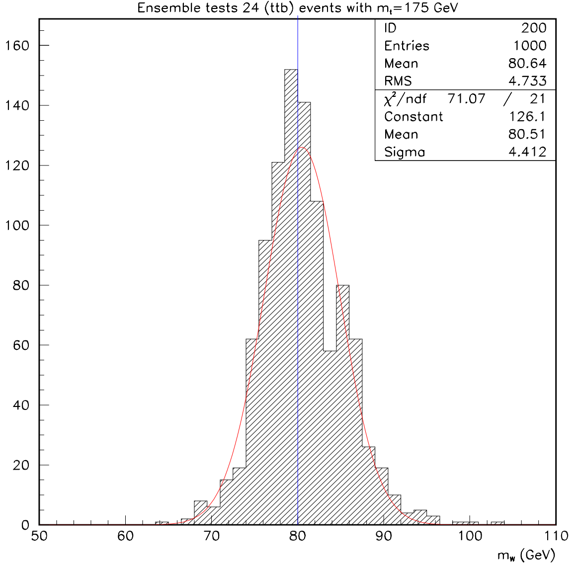
Figure 7.10: Ensemble tests for the determination of the mass of the W boson in the hadronic branch of the t\bar{t} event. Each experiment is simulated using 24 signal t\bar{t} events and no background, with M_t = 175 GeV.
