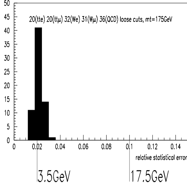
Figure 7.7: Esemble test with Sample 2. The displayed statistical error is obtained from the width of the likelihood for each experiment.
