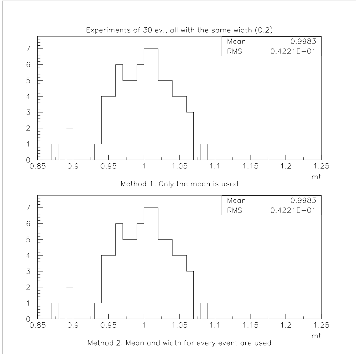
Figure A.1: Histograms of estimators of \langle x \rangle obtained from 80 samples of 30 events using Method I (top) and Method II (bottom). All events have the same width for their probability distributions. As expected, the plots show no difference between these two procedures.
