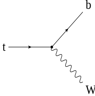
Figure 2.3: Decay of the top ( t ) quark into a W boson and a bottom ( b ) quark.
