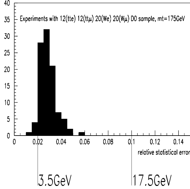
Figure 7.5: Ensemble test with Sample 1. The displayed statistical uncertainty is obtained from the width of the likelihood for each experiment.
