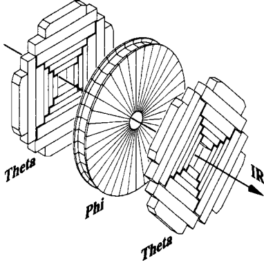
Figure 3.5: Schematic of the FDC. Two \Theta modules with a \Phi module in between.
