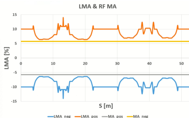
Figure 6. Momentum acceptance for RFMA and LMA.
