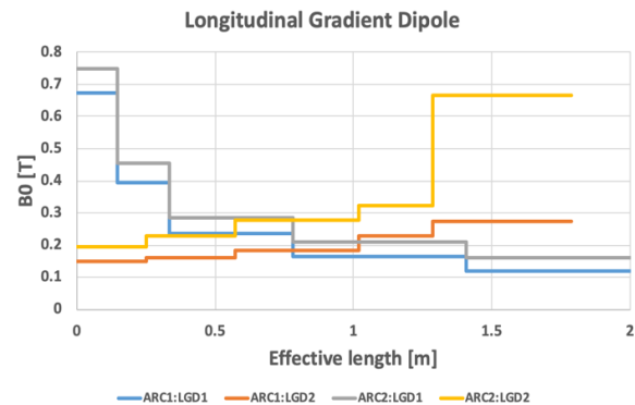
Figure 4: Longitudinal gradient dipole field strength of LGD1 and LGD2 for ARC1 and ARC2.
