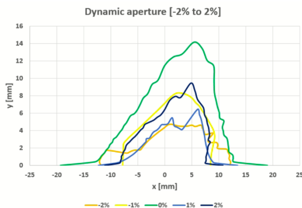
Figure 5. An optimized dynamic aperture of 4GSR.
