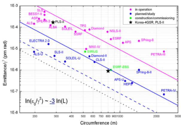
Figure 1. Distribution of performance according to storage ring circumference of 3rd generation light source and 4GSR.
