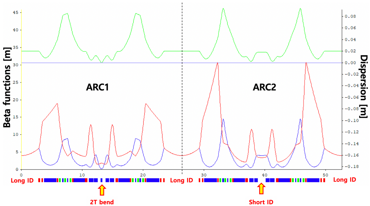
Figure 3: Twiss parameters of combined 4GSR HMBA lattice. The designed natural emittance is 53 pm rad.
