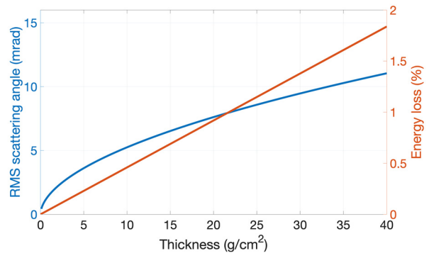
Figure 4: The RMS scattering angle and energy loss for 2.5 GeV protons interacting with different thickness of tantalum.
