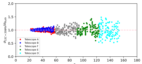
Figure 5. \sigma_{12\text{C}}/\sigma_{\text{Ruth}} angular distribution geometrically optimized and corrected by electronic efficiency.
