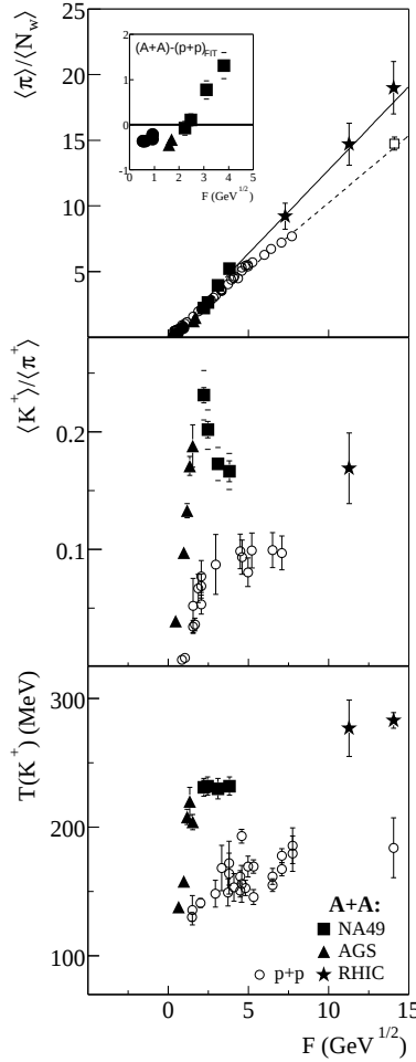
Fig. 1. Collision energy dependence ( F \equiv (\sqrt{s_{NN}} - 2m_N)^{3/4} / \sqrt{s_{NN}}^{1/4} \approx s_{NN}^{1/4} , where m_N is nucleon mass) of various hadron production properties (for details see text) measured in central Pb + Pb and Au + Au collisions (solid symbols) compared to results from p + p reactions (open dots). The changes in the SPS energy range (solid squares) suggest the onset of the deconfinement phase transition.
