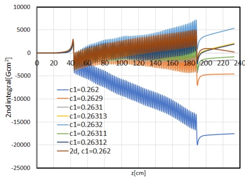
Figure 7: The 2 nd integral ( \text{G cm}^2 ) at C1 = 0.262 to 0.2632 based on the 3D model and optimal case from the 2D model ( C1 = 0.262 , C2 = 0.75 ).
