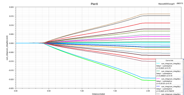
Figure 6: The 2 nd field integrals calculated by the 2D optimizer with both C1 and C2 as variables, C1 = 0-1 and C2 = 0-1.
