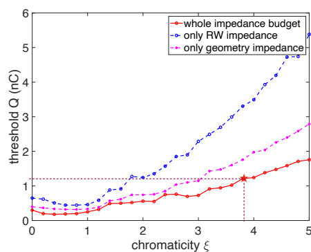
Figure 6: Single-bunch vertical instability threshold (without HHC) as a function of the vertical chromaticity including resistive-wall impedance only (blue line), geometry impedance only (magenta curve) and total impedance budget (red curve).
