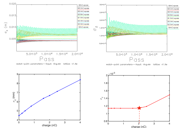
Figure 4: Single-bunch longitudinal dynamics simulations without HHC indicate ~2 nC/bunch threshold for the onset of a micro-wave instability. The four figures show the rms bunch length revolution (top left), energy spread revolution (top right), rms bunch length (bottom left) and rms. energy spread (bottom right) vs. bunch charge.
