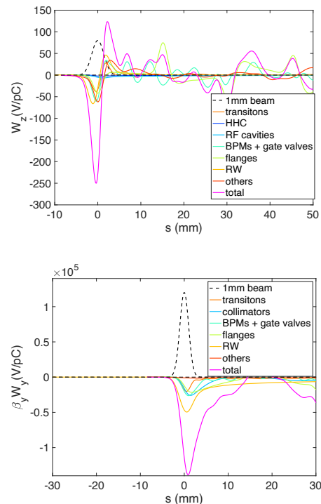
Figure 1: Longitudinal (top) and vertical (bottom) pseudo-wake functions for the various sources, as indicated in the in-set, and their total (1 mm long rigid drive bunch).
