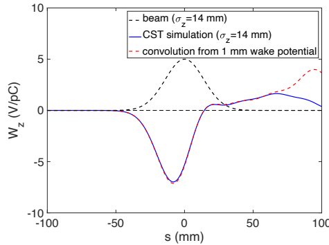
Figure 2: Consistency check of the calculation for the wake potential of a 14 mm bunch based on the longitudinal pseudo-Green function vs. a direct calculation in CST.
