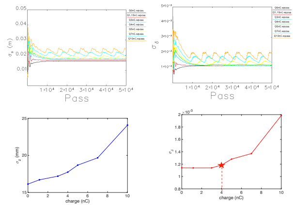
Figure 3: Single-bunch longitudinal dynamics simulations with HHC indicate ~4 nC/bunch threshold for the onset of a saw-teeth instability. The four figures show the rms bunch length revolution at different charge (top left), rms bunch energy spread revolution at different charge (top right), rms bunch length (bottom left) and rms energy spread (bottom right) vs. bunch charge after about 2.5 damping times.
