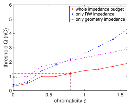
Figure 5: Single-bunch vertical instability threshold (with HHC) as a function of the vertical chromaticity including resistive-wall impedance only (blue line), geometry impedance only (magenta curve) and total impedance budget (red curve).
