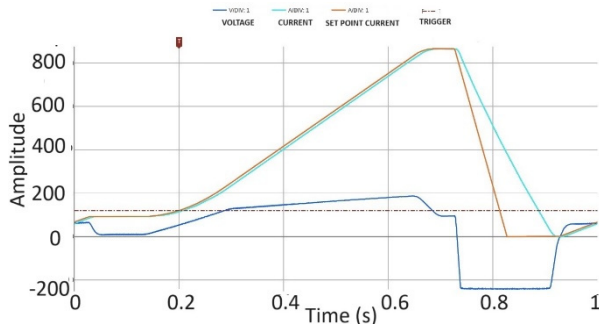
Figure 4: Booster dipole PS ramp.
