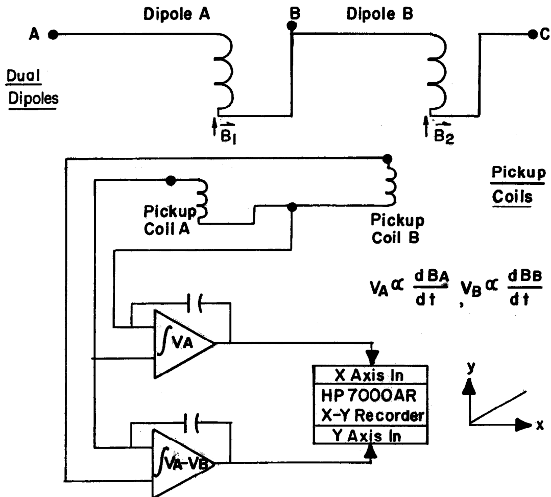
Figure 5 Dual Dipole Tracking Test-Instrumentation
