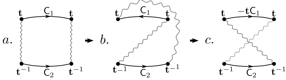
Figure 3.3: a. Two cuts and two basis contours for a four-punctured sphere. b. The result of the braiding transformation. c. We moved the contour C_1 across the cut and reversed its orientation, which produced a factor of -\mathbf{t} .
