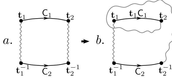
Figure 3.16: a. Two cuts and two basis contours for a four-punctured sphere. b. The result of the braiding transformation. The contour C_1 got multiplied by t_1 in crossing the left cut. It will also get a factor of t_2 , when the right cut is moved back to its place.
