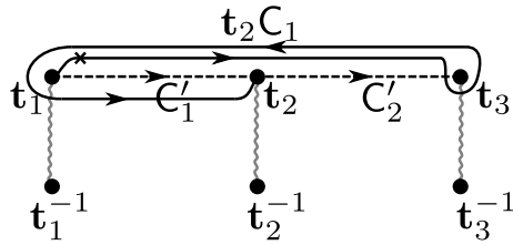
Figure 3.20: Contour t_2 C_1 , which comes from C_1 of fig. 3.19 after moving the middle cut back to its place. We show the new basis contours C'_1 and C'_2 by dashed lines.
