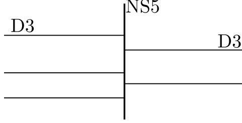
Figure 2.1: An NS5-brane with m D3-branes ending on it from the left and n from the right – sketched here for m = 3 , n = 2 . The D3-branes but not the NS5-brane extend in the x_3 direction, which is plotted horizontally, and the NS5-brane but not the D3-branes extend in the x_{4,5,6} directions, which are represented symbolically by the vertical direction in this figure.
