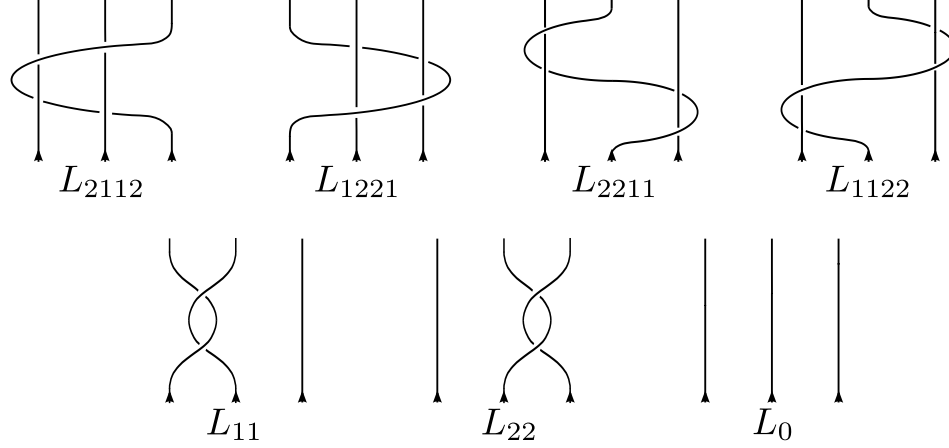
Figure 3.18: Braids for the 3-strand skein relation.
