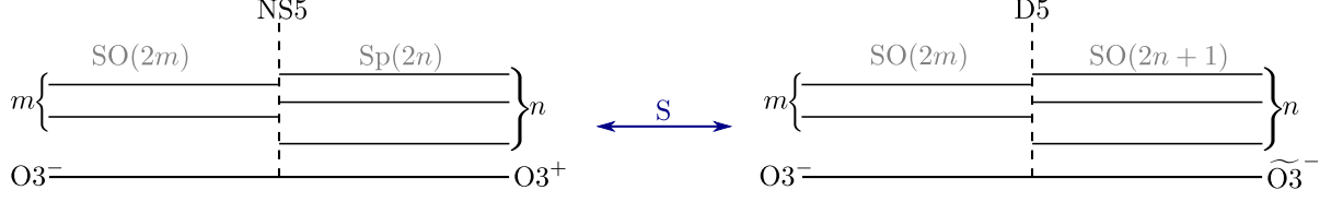
Figure 2.9: The brane configurations that realize the electric and magnetic theory for the four-dimensional construction of the \mathrm{OSp}(2m|2n) Chern-Simons theory.
