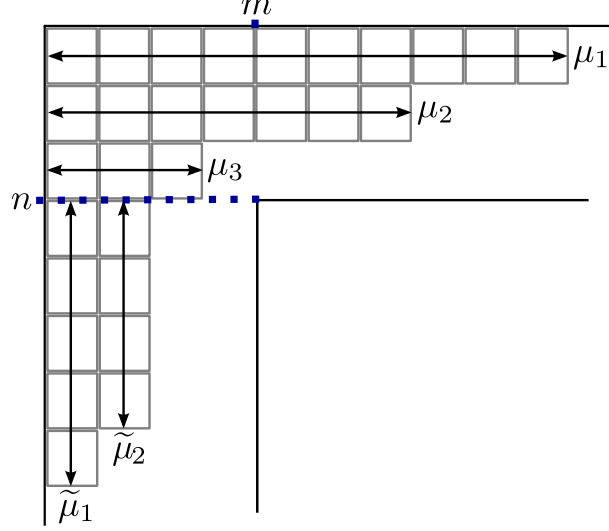
Figure 2.12: Example of a hook partition for \mathfrak{osp}(9|6) . The labels \mu_i , i = 1, \dots, n and \tilde{\mu}_j , j = 1, \dots, m were defined in (2.202). Here \mu_3 = 3 , and, clearly, no more than the first three \tilde{\mu} 's can be non-zero.
