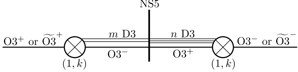
Figure 3.11: The brane construction for the \mathcal{N} = 4 Gaiotto-Witten theory, which upon twisting would give \text{OSp}(2m|2n) Chern-Simons. The leftmost and rightmost orientifold planes are O3^\pm , if k is even, and \widetilde{O3}^\pm , if k is odd.
