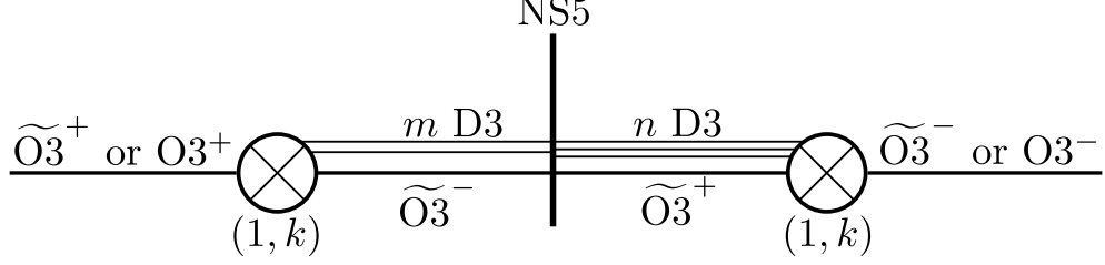
Figure 3.10: The brane construction for the \mathcal{N} = 4 Gaiotto-Witten theory, which upon twisting would give \text{OSp}(2m+1|2n) Chern-Simons. The leftmost and rightmost orientifold planes are \widetilde{\text{O3}}^\pm , if k is even, and \text{O3}^\pm , if k is odd.
