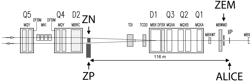
Figure 1.23: Schematic top view of the ALICE beam line opposite to the muon spectrometer. The locations of the neutron (ZN), proton (ZP) and forward electromagnetic calorimeters (ZEM) are shown.
