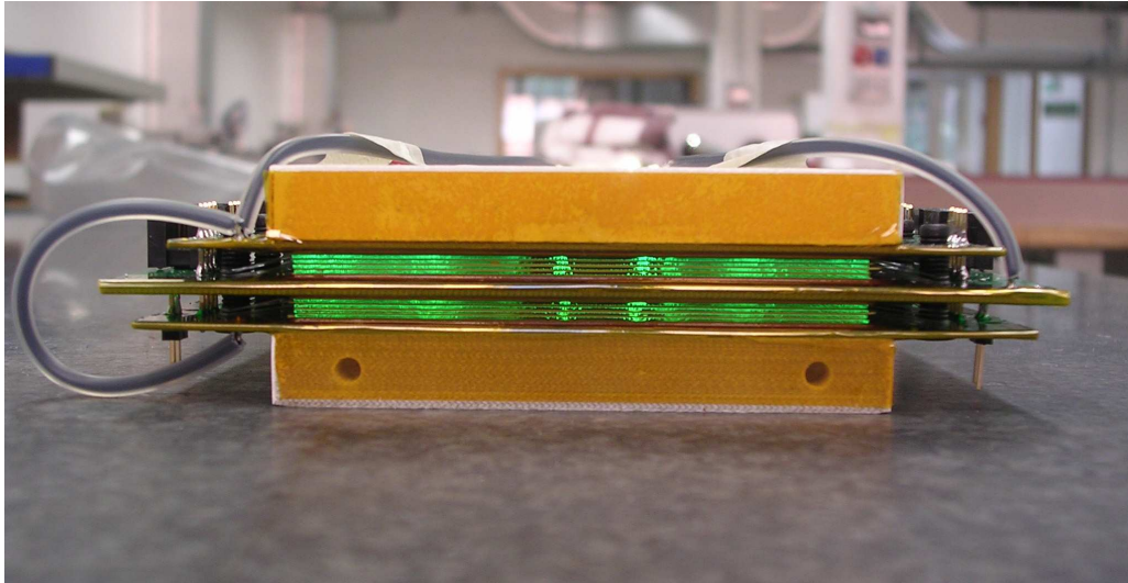
Figure 2.7: Photograph of a 10-gap double-stack MRPC strip.
