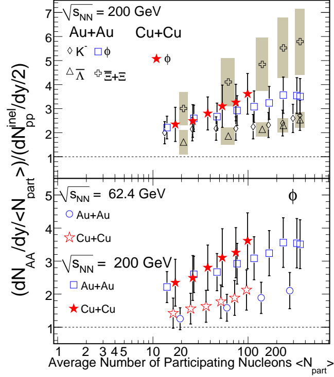
Figure 1.6: Strangeness enhancement measured by the STAR experiment. Upper panel: the ratio of the yields of K^- , \phi , \bar{\Lambda} and \Xi + \bar{\Xi} normalized to \langle N_{part} \rangle in nucleus–nucleus collisions and to corresponding yields in inelastic pp collisions as a function of \langle N_{part} \rangle at 200 GeV. Lower panel: same as above for \phi mesons in Cu–Cu collisions at 200 and 62.4 GeV.
