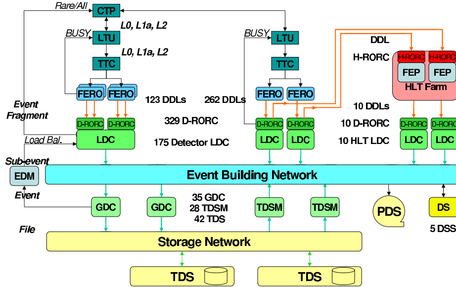
Figure 1.26: The overall architecture of the ALICE DAQ system and the interface to the HLT system.
