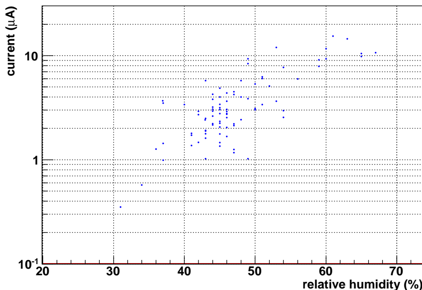
Figure 3.10: Module current measured during high-voltage test in air at \pm 3 kV as a function of the relative humidity.
