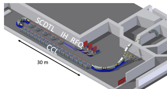
Figure 5: Sketch of CABOTO all-linac solution (courtesy of M. Vaziri—TERA Foundation)
