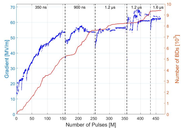
Figure 4: Conditioning history of the first BTW prototype, tested at CERN Sbox [25].
