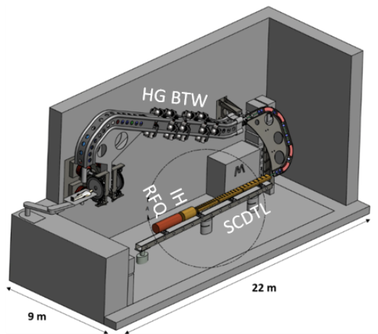
Figure 3: Sketch of TULIP all-linac solution (courtesy of M. Vaziri—TERA Foundation).
