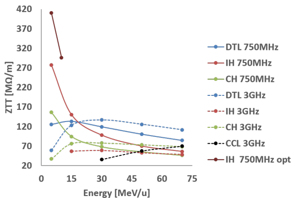
Figure 2: ZTT as a function of the RF cavity energy for different low energy RF cavities [12].
