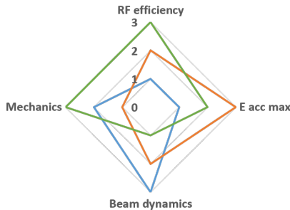
Figure 1: Qualitative assessment between RFQ, DTL and H-type cavities for low energy acceleration. RFQ in blue, DTL in orange, H-type cavities in green.
