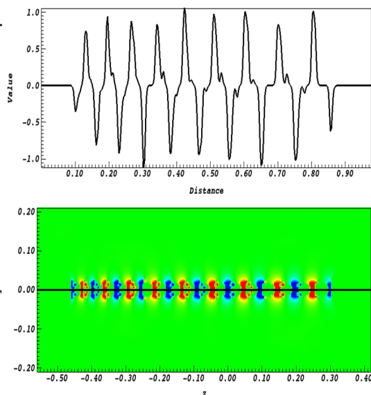
Figure 4: Electric field amplitude along the longitudinal axis for the RFI at the operating mode.
