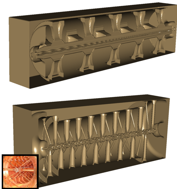
Figure 2: VSim 9 models of the RFQ (top) and the RFI (bottom). The inset is an image of the actual RFI cross section.
