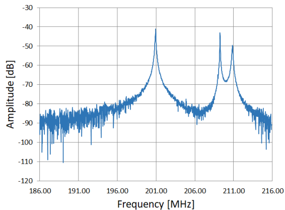
Figure 5: Mode spectrum for the RFQ; fundamental mode is close to 200 MHz and parasitic modes in the neighborhood of 210 MHz.
