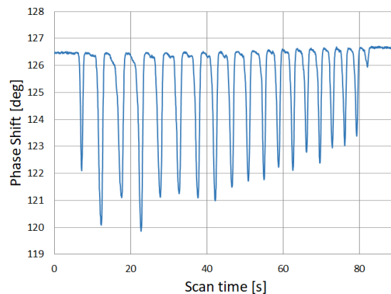
Figure 6: Bead-pull measurement data showing phase shift vs. scan time along the RFI axis.
