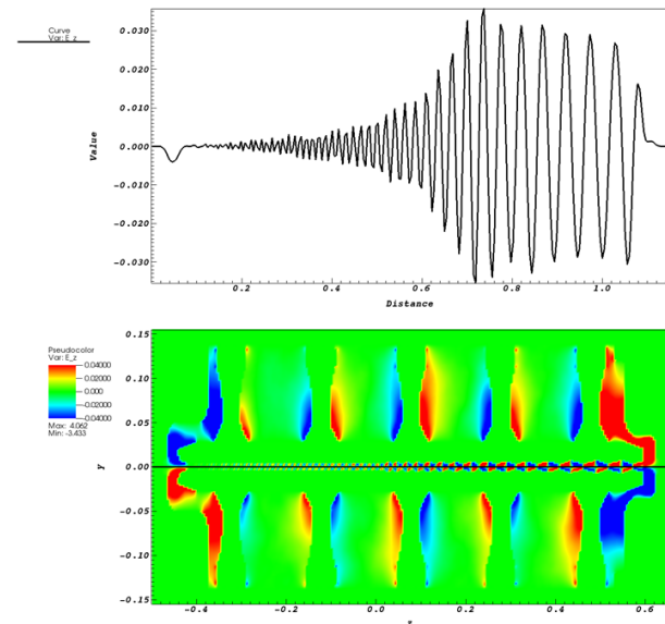
Figure 3: Amplitude of the longitudinal electric field corresponding to the operating mode at 200 MHz of the RFQ.
