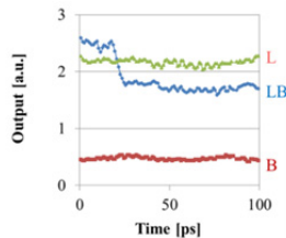
Figure 3: Bolometer output as a function of the optical delay for the probe (OD2). LB, L, and B denotes the shutters (S1/S2) conditions for front/back electron beams of Opened/Open, Opened/Closed, and Closed/Open, respectively. The transient decrease in transmittance was observed at a time of \sim 20 ps.
