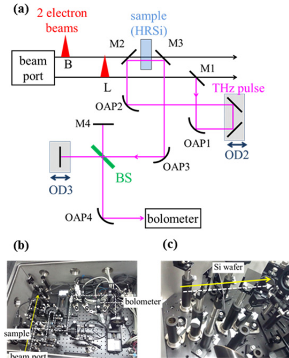
Figure 2: (a) Pulse radiolysis using THz probe pulses. Beams of “L” and “B” were used for generation of THz probe pulses and irradiation of a sample, respectively. OAP: an off-axis parabolic mirror, M denotes a plane mirror, and BS denotes a beam splitter. (b) Picture of a low-vacuum chamber. Lines denote paths of beams and probes. (c) Picture of the sample irradiated by the pump beam (B, solid line) and path of the beam for the probe-generation (L, dashed line).
