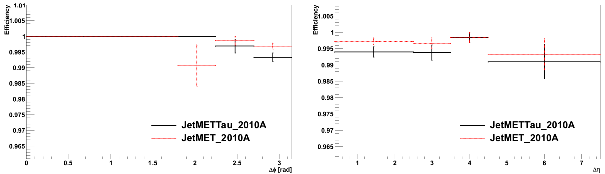
Figure 5.4: Efficiency of the trigger combination for the inside-jet veto scenario in the JetMET-Tau_2010A (solid black line) and JetMET_2010A datasets (dashed red line). The trigger efficiency as a function of \Delta\phi is presented on the left side and as function of \Delta\eta on the right side.
