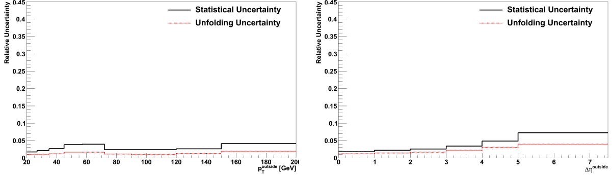
Figure 7.4: Relative statistical (black–solid) and unfolding (red–dashed) uncertainties of the leading outside–jet p_T (left) and \Delta\eta^{out} (right) distributions.
