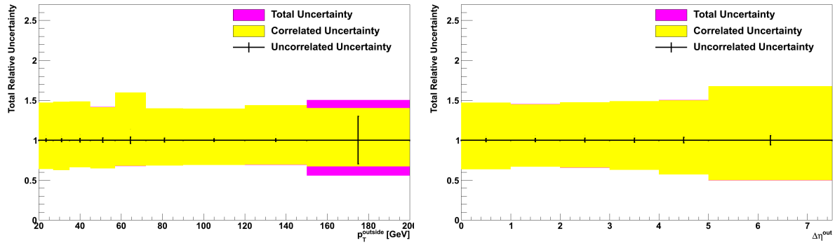
Figure 7.23: Relative total uncertainty of the outside-jet p_T (left) and \Delta\eta^{\text{out}} (right) distributions.
