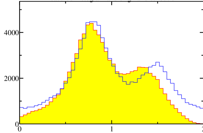
Figure 6.1: Example of true (blue) and measured distributions (red and yellow filled area) [175].
