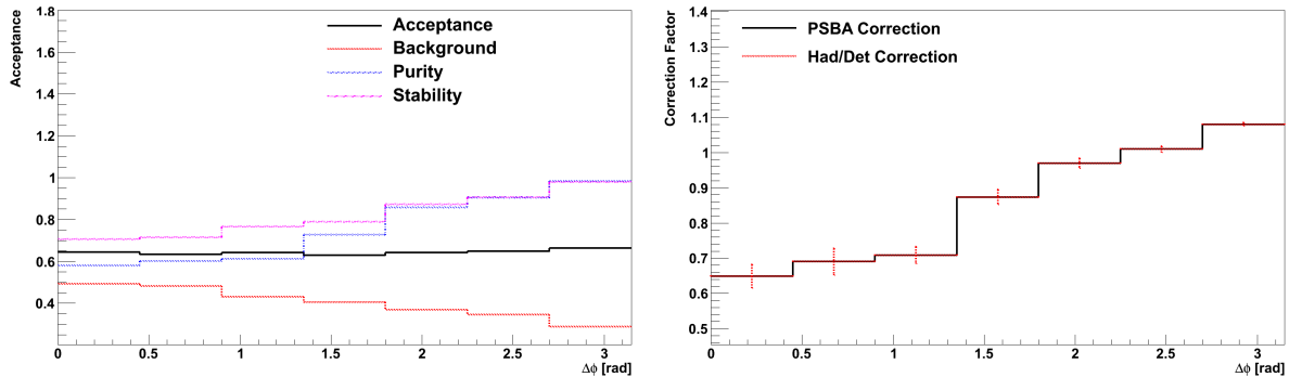
Figure 5.33: Acceptance, background, purity and stability (left) and closure test (right) for the bin-by-bin correction performed on the JetMETTau_2010A datasample corrected with PYTHIA 6 - Z2* Tune in the inclusive scenario.
