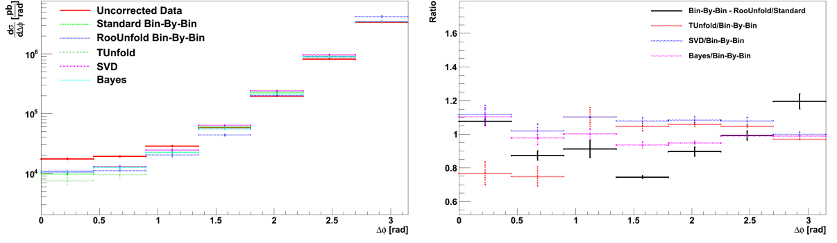
Figure 6.16: PYTHIA 6 Z2* tune on detector level unfolded with PYTHIA 8 4C tune response matrix for \Delta\phi in the inclusive scenario for the JetMETTau_2010A dataset. Cross-section (left) and ratio (right). The PYTHIA 6 Z2* tune on detector level is represented with a red line, denoted as uncorrected data. The MC truth is labeled as standard bin-by-bin and is represented with a green line. The other curves represent the unfolding results.
