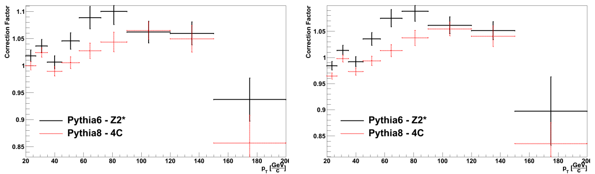
Figure 5.45: Correction factors to stable particle level for leading outside-jet p_T for the JetMET-Tau_2010A (left) and JetMET_2010A (right) datasets.
