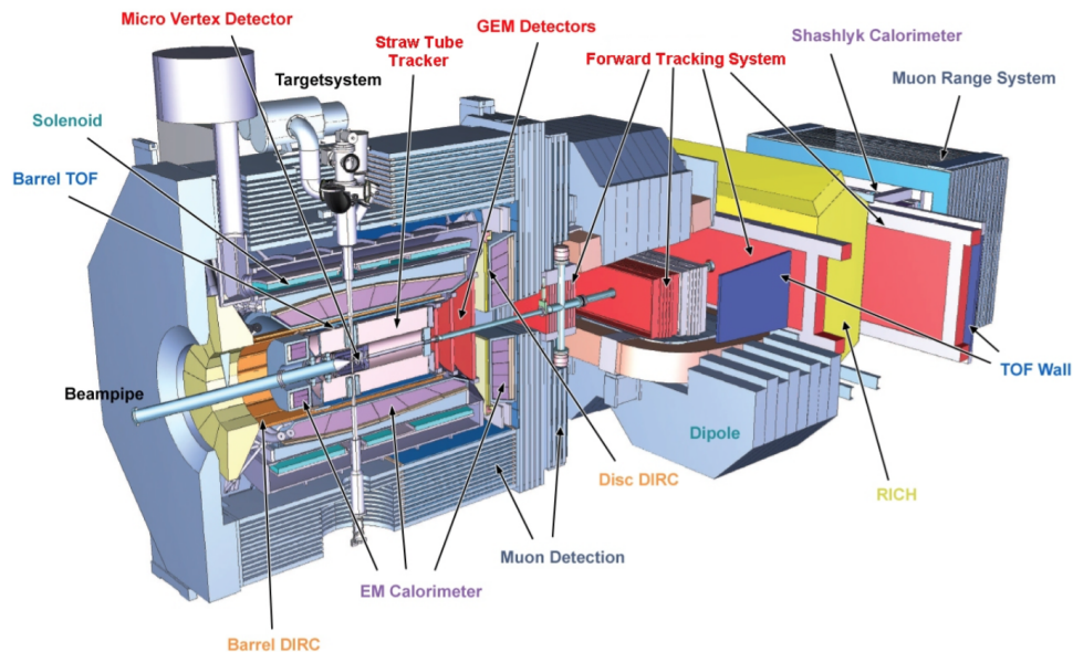
Figure 1. The \bar{P} ANDA detector setup.
