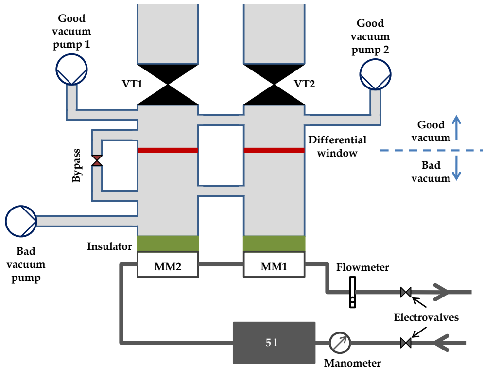
Figure 3.12: Scheme of the vacuum system and gas system for Sunset Micromegas detectors.
