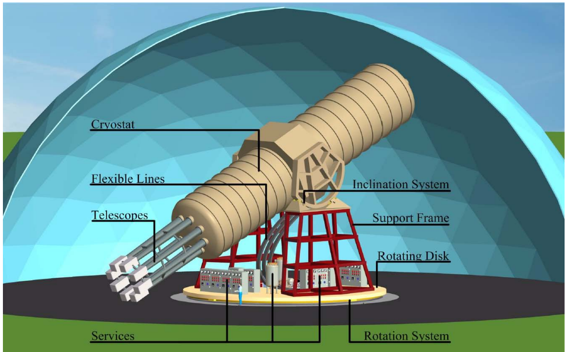
Figure 8.2: Schematic view of the IAXO proposal. The different parts of the magnet, magnet support and feeds are labeled. Plot taken from [135].
