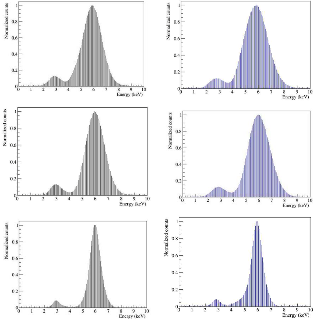
Figure 5.2: Normalized spectra for a set of calibrations. Different detectors are shown: Sunсет1 on the top, Sunсет2 on the middle and Sunrise in the bottom. The plots on the left show the spectra of the mesh (black bars) while the plots on the right side correspond to the spectra in the strips readout.
