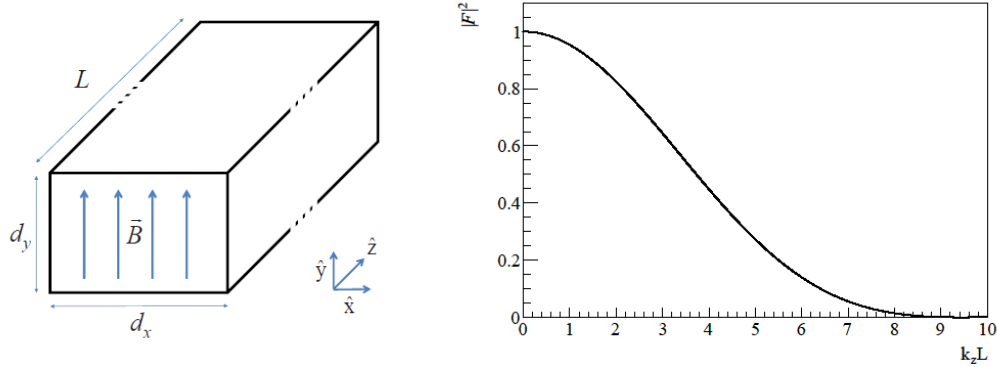
Figure 9.1: Left: Sketch of the cavity geometry used for the calculations. Right: |F|^2 versus k_z L for a single incoming axion momentum k as expressed in equation 9.5. Plots taken from [142].
