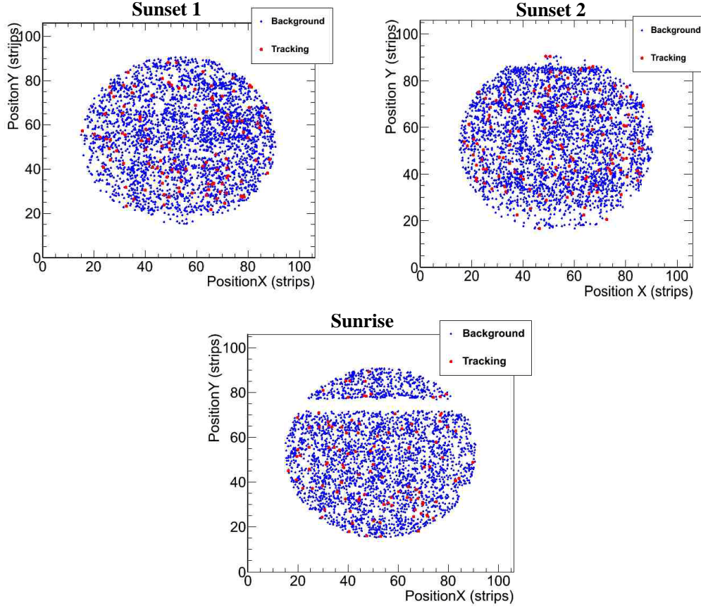
Figure 5.10: Spatial distribution of the background (blue dots) and tracking (red dots) events during the 2011 data taking campaign. Only the events inside the coldbore area and inside the RoI [2 - 7] keV are shown.
