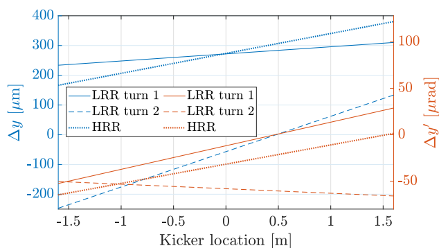
Figure 2: Vertical separation in position and angle between camshaft and main beam at the center of the BL17 undulator with a PSB kick angle of 85 \mu\text{rad} . Kicker location z = 0 refers to the midpoint of the long straight section.
