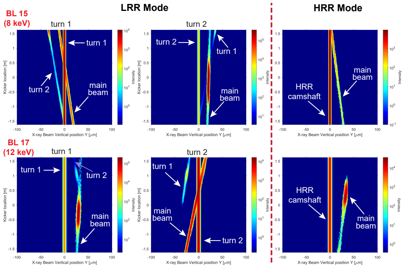
Figure 5: X-ray beam profiles (horizontal axis) at the focal plane of BL15 and BL17 as a function of PSB kicker location (vertical axis). First two columns represent profiles at LRR operation and mono slits aligned to turn 1 or turn 2 camshaft beam. Third column represents profiles at HRR operation and mono slits aligned to the camshaft beam.
