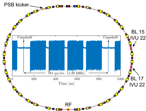
Figure 1: Layout of SPEAR3 lattice. PSB kicker and undulators for two beamlines (BL15 and BL17) used in this work are highlighted. Inset shows the typical fill pattern in SPEAR3 with a camshaft bunch sitting in the middle of two bunch trains with a \sim 120 -ns gap.
