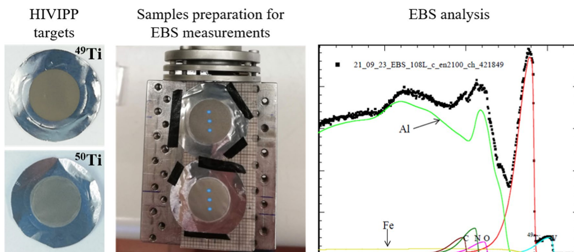
Fig. 1 Enriched target manufacturing and characterization at the INFN-LNL. The blue dots in the center photo represent the positions where the EBS scans were performed to assess the thickness homogeneity along the diameter. (Color figure online)
