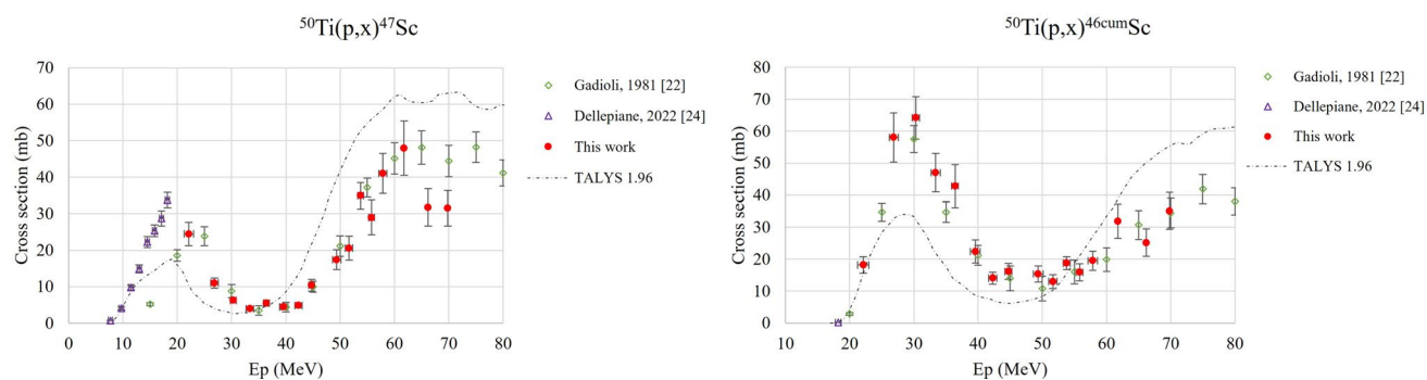
Fig. 4 The ^{50}\text{Ti}(p,x)^{47}\text{Sc} (left) and ^{50}\text{Ti}(p,x)^{46\text{cum}}\text{Sc} (right) cross section
