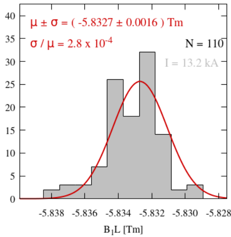
Figure 3: Distribution of the measured magnetic length at a current of I = 13.2 kA of 110 dipole magnets.
