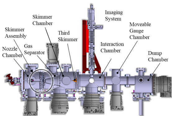
Figure 2: Gas jet monitor used for fluorescence-mode R&D.
