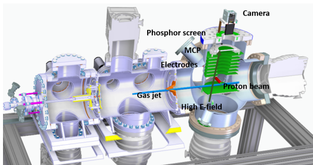
Figure 5: Test gas jet profile system designed for measurements at the University of Birmingham MC40 cyclotron.
