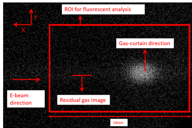
Figure 3: Example gas jet profile image from the system presented in Fig. 2.
