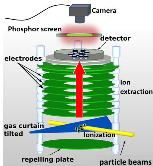
Figure 1: A schematic demonstrating the operating principle of the gas jet profile monitor.
