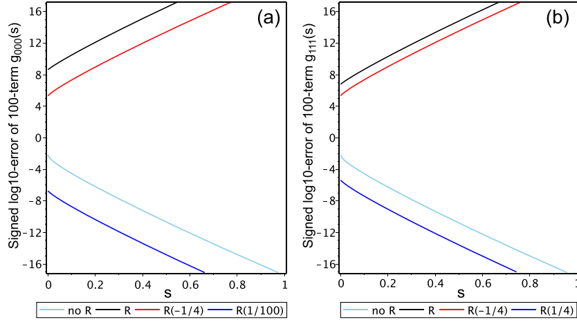
Figure 4. Error in evaluation of LGF for the simple cubic lattice at (a) origin and (b) point (1, 1, 1) by path expansion with different \epsilon_{\text{up,low}} - \epsilon_{\infty} (shown in parentheses) in the remainder (24).
