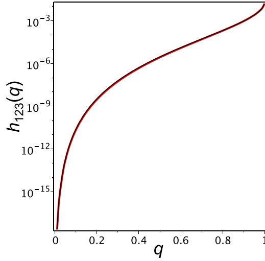
Figure 2. Large-scale approximation (red curve versus exact-LGF black curve) for simple cubic lattice is accurate even for small values of coordinates, x = (1, 2, 3) . The argument q is defined by equation (14).
