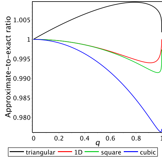
Figure 5. Lerch transcendent approximation to Green's function of several lattices at origin. Here \varepsilon is determined by the first path expansion coefficient (e.g. \varepsilon = 2^{2/d}d/2\pi for hypercubic lattices).
