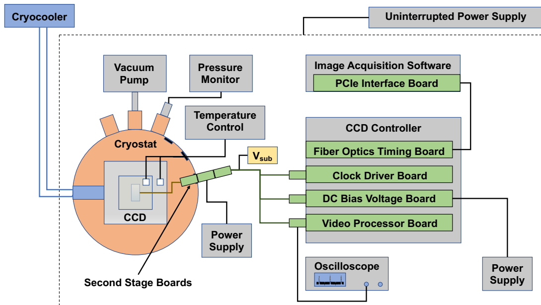
Figure 5.1: Schematic of an automated CCD test chamber at LPNHE, Paris.
