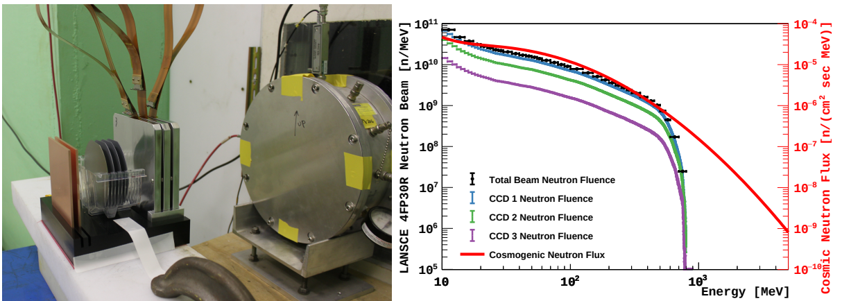
Figure 3.15: Left: Layout of CCDs and wafers irradiated at the LANSCE neutron beam. Right: Comparison of LANSCE beam fluences with sea-level cosmic-ray neutrons [87].
