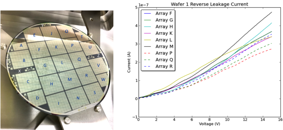
Figure 2.21: Left: labeled arrays of wafer W1; Right: corresponding leakage current profiles.
