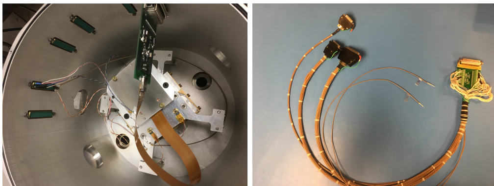
Figure 5.4: Left: A 4k \times 2k CCD installed in the LPNHE setup and secured to a UW second stage board. Right: The Medusa cable used to deliver clock, bias, and video lines.
