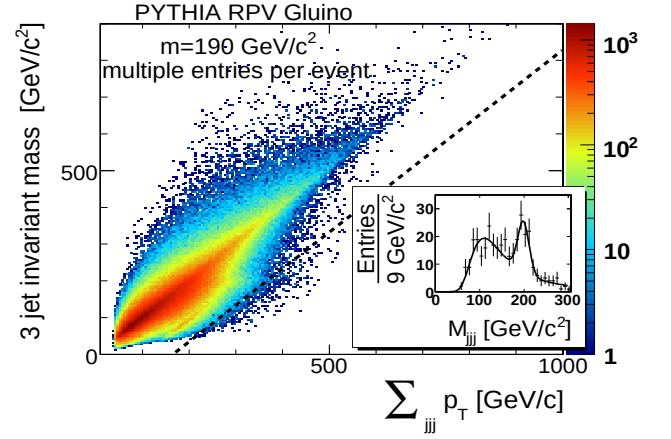
FIG. 1. Distribution of M_{jjj} versus \sum_{jjj} p_T for a pair-produced RPV gluino with invariant mass 190 GeV/c 2 generated with PYTHIA MC. Triplets to the right of a diagonal offset ( \sum_{jjj} p_T - M_{jjj}c = \Delta ), indicated by the dashed line, are kept. The inset shows the M_{jjj} distribution for the RPV signal MC and with no QCD background after a diagonal offset of 195 GeV/c along with a Gaussian plus a Landau fit; the Landau shows the combinatorial contribution within the signal jet ensemble. The QCD background distribution resembles that of the combinatorial contribution, because they are both due to effectively uncorrelated triplets.
