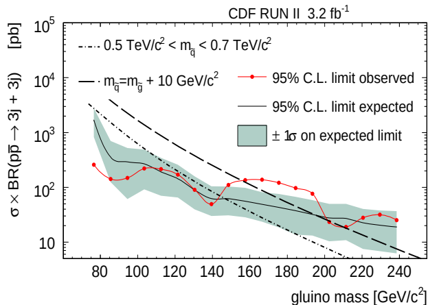
FIG. 3. The observed (points) and expected (solid black line) 95% confidence level limits on the production cross section \sigma(p\bar{p} \rightarrow XX') \times \text{BR}(\tilde{g}\tilde{g} \rightarrow 3 \text{ jet} + 3 \text{ jet}) where X, X' = \tilde{g}, \tilde{q}, or \tilde{\bar{q}} , including systematic uncertainties. The shaded bands represent the total uncertainty on the limit. Also shown is the model cross section from PYTHIA corrected by an NLO k -factor (dash-dot line for 0.5 \text{ TeV}/c^2 < m_{\tilde{q}} < 0.7 \text{ TeV}/c^2 , dashed line for m_{\tilde{q}} = m_{\tilde{g}} + 10 \text{ GeV}/c^2 ).
