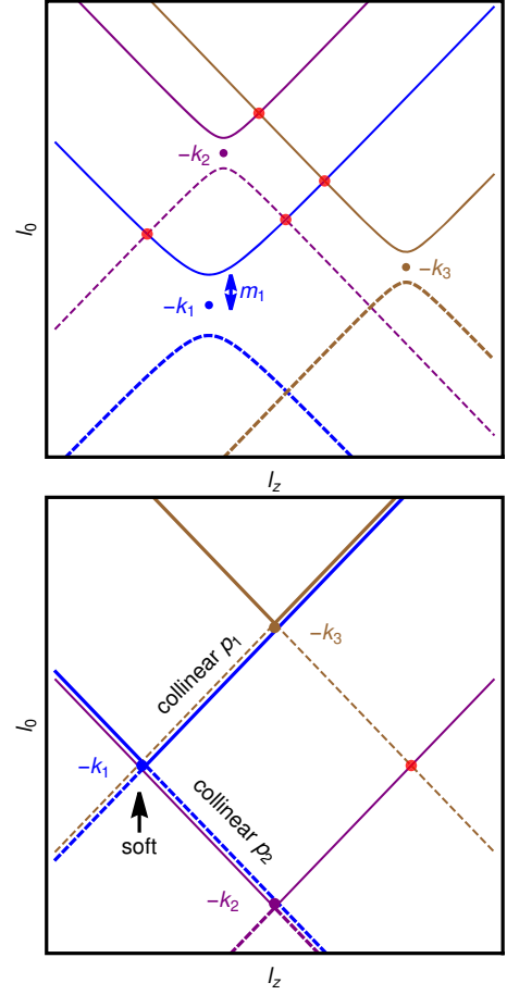
Figure 1: On-shell hyperboloids for three arbitrary propagators in Cartesian coordinates in the (\ell_0, \ell_z) space (up). Kinematical configuration with infrared singularities (down). In the latter case, the on-shell hyperboloids degenerate to light-cones.
