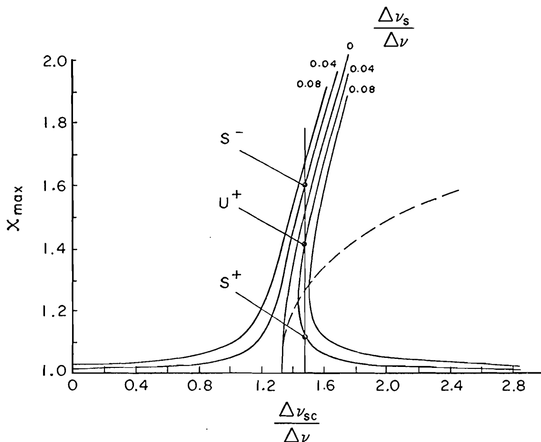
Fig. 8. Response diagram: x_{\max} = \left( \sqrt{1 + A^2} + A \right)^{\frac{1}{2}} . The curves to the left of \frac{\Delta \nu_s}{\Delta \nu} = 0 correspond to the upper sign in Eqs. (2-15) and (2-16); those to the right correspond to the lower sign. The points where the slope is vertical (indicated by the dashed curve) are referred to as critical points.
