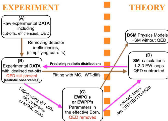
Fig. 3. Scheme of construction of EWPOs at FCC-ee. Main difference with LEP is Monte Carlo use in steps (B)→(C) and (B)→(D) instead of programs like ZFITTER/TOPAZO.
