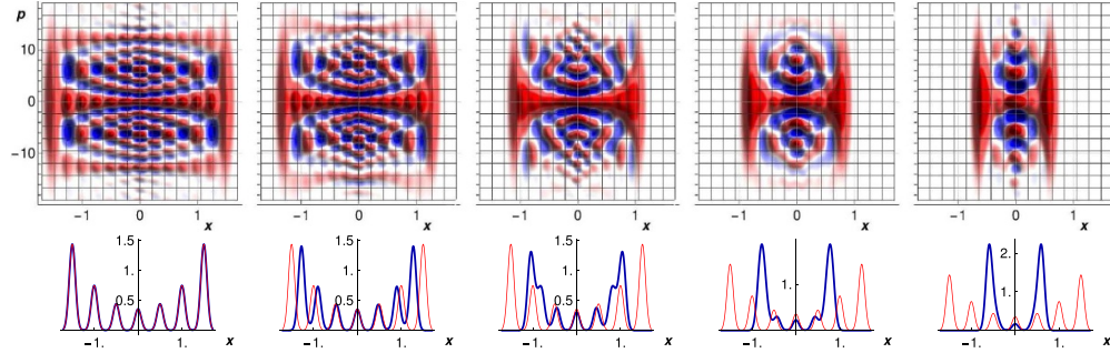
Figure A.16. ‘Double eye’ pattern in phase space: similar to figure A.15, but for an odd number of peaks, yielding positive (red) centres in W(x,p) . Inter-peak phase differences are zero whereas distances are not constant.
