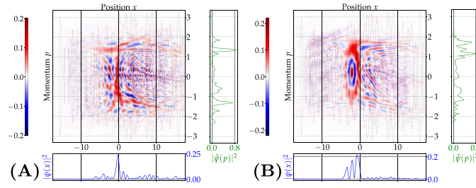
Figure 7. Random comb-states form in a random potential giving rise to lines across phase space and the formation of ‘eye’ patterns.
