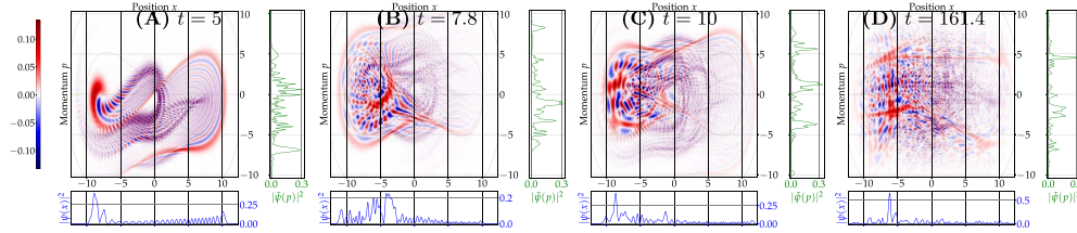
Figure 2. Wigner distributions evolved in double well potential V(x) = x^4/200 - x^2/2 . The initial state \psi_0 = (2/5\pi)^{1/4} \exp[-(x+9.9)^2/5] has an energy that partly exceeds the central barrier as can be seen clearly at short times (A). Subsequently, lines form quite soon (B) and keep reappearing (C)–(D).
