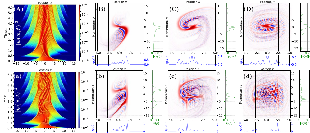
Figure 10. Enhanced line formation with attractive interaction: The initial state \psi_0(x) = 0.43 \exp[-(x-2)^2/19] evolves in the potential V(x) = \frac{1}{10}x^4 without, ( \gamma = 0 ) top row ((A)–(D)), and in the presence of attractive interaction ( \gamma = 50 and \epsilon = 2 ) bottom row ((a)–(d)). The spatial probability density |\psi(x, t)|^2 , (A) and (a), shows dynamics dominated by oscillations due to the potential’s confining forces. The associated Wigner distributions (using the same colouring as in figure 8), at times (B) and (b) t = 0.55 , (C) and (c) t = 1.76 , and (D) and (d) t = 4.52 , prominently display straight lines crisscrossing phase space for the nonlinear case (b)–(d) whereas only weak lines form in the linear case, also see appendix ‘Repulsive nlse’ .
