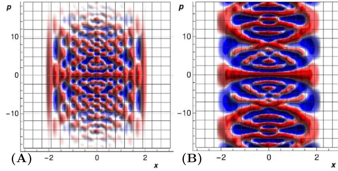
Figure 4. (A) W of comb-state versus (B) \mathcal{I} of equation (4), with \Lambda = 1 , with same locations and weights of peaks of comb-state as in figure 6(E). Both representations yield similar interference patterns: we conclude that coherences between peaks in comb-states are responsible for formation of lines.
