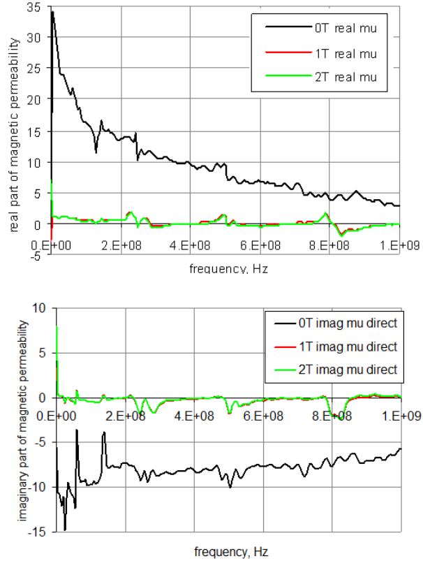
Figure 4: Calculated magnetic permeability of steel in magnetic field, parallel to strip plane.
