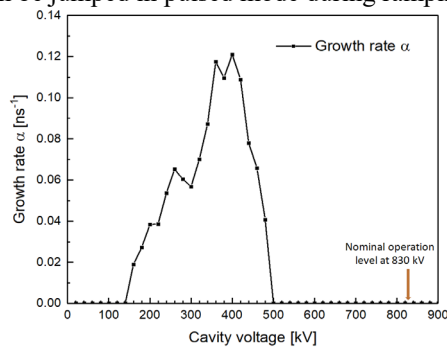
Figure 4: Exponential growth rate \alpha as a function of the gun voltage.
