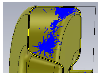
Figure 3: Stable multipacting trajectories at 400 kV cavity voltage in the gun, one point 1 st order MP.
