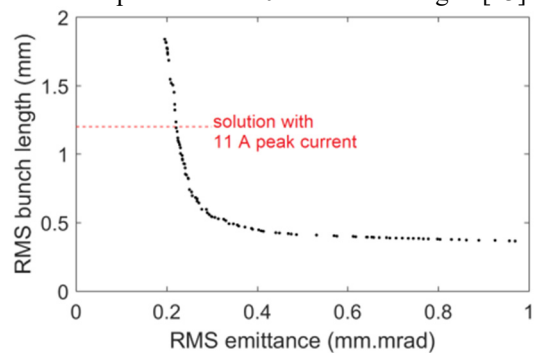
Figure 6: Pareto front of 100 pC beam with 1 mm.mrad/mm thermal emittance, 10k macro-particles simulations.
