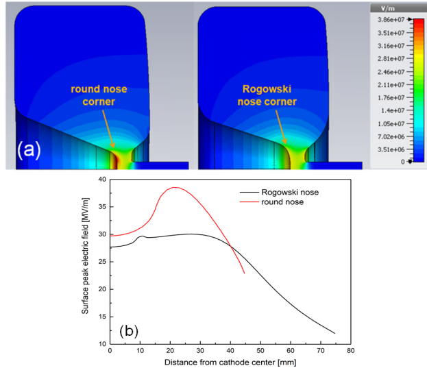
Figure 1: Electric field distribution with an input power of 100 kW. (a) Cavity with round cathode nose (left), cavity with Rogowski profile cathode nose (right); (b) surface field comparison along the cathode nose curve.
