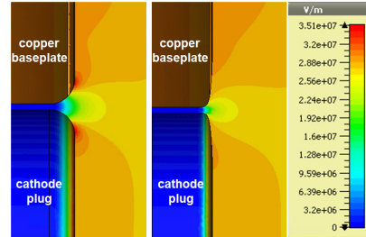
Figure 2: Field map in the cathode plug vicinity. Left: round corner; right: Rogowski corner.
