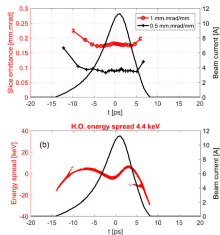
Figure 7: Refined simulation with 250k macro-particles, 100 pC with 11 A peak current, (a) slice emittance with two thermal emittance settings, (b) longitudinal phase space after removing the 1 st and 2 nd order chirps, the higher order energy spread is 4.4 keV.
