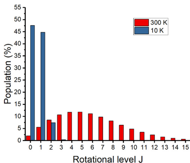
Figure 5. The rotational level population of BaH + in the ground electronic and vibrational state at 300 K (red), and 10 K (blue) at thermal equilibrium.
