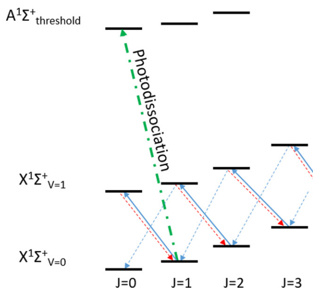
Figure 6. A mid infra-red laser drives \Delta J = -1 transitions (solid blue) from the ground to the first excited vibrational level of BaH + . The level can then decay back to the ground vibrational level via a \Delta J = -1 transition (dashed blue), achieving rotational cooling, or via a \Delta J = +1 transition (dashed red) to the state of origin. The photodissociation transition is shown in green.
