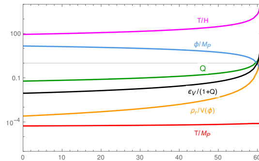
Figure 3. Evolution of the different quantities in the WI scenario for the case of V(\phi) = \frac{1}{2}m^2\phi^2 , Y = C_T T , with m = 10^{-7}M_{Pl} and C_T = 0.002 .
