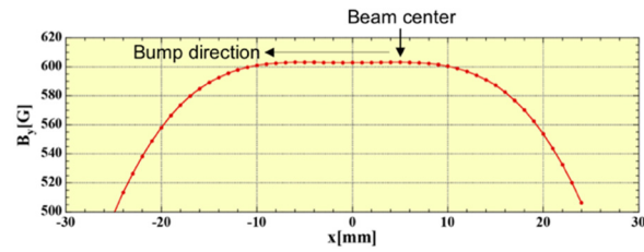
Figure 6: Horizontal distribution of the measured vertical magnetic field at the center of BMIS02 for I_{BMIS02} = 4.67 A.
