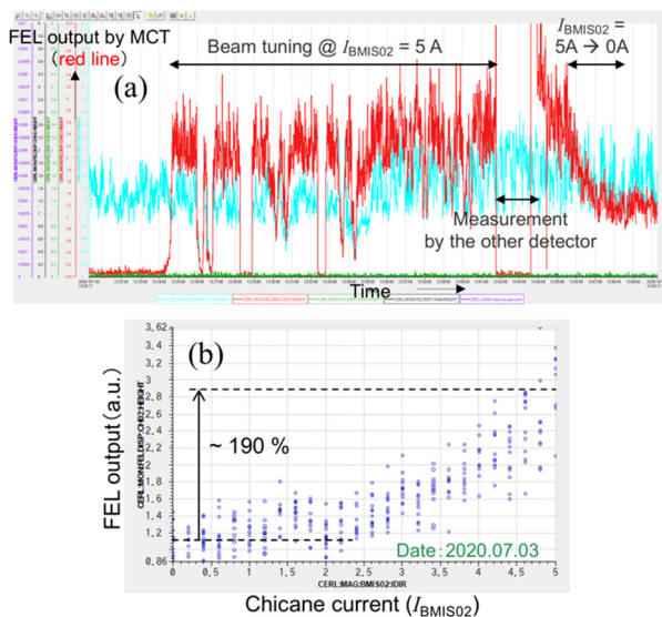
Figure 9: (a) Time chart and (b) chicane-current dependence of the FEL output measured by the MCT detector in 3 rd July 2020.
