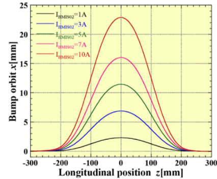
Figure 5: Calculated closed bump orbits made by the chicane magnet for I_{BMIS02} = 1, 3, 5, 7, 10 A with R = 0.8357 .
