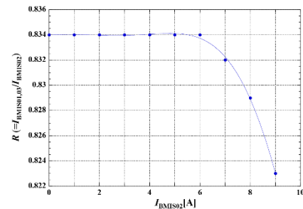
Figure 7: Current ratio of the chicane magnet as a function of I_{BMIS02} for making the bump orbit closed and the fitted sixth-order polynomial curve.
