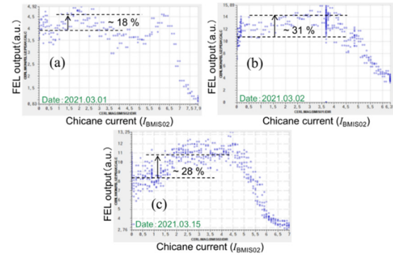
Figure 10: Chicane-current dependences of the FEL output in (a) 1 st , (b) 2 nd , and (c) 15 th March 2021.
