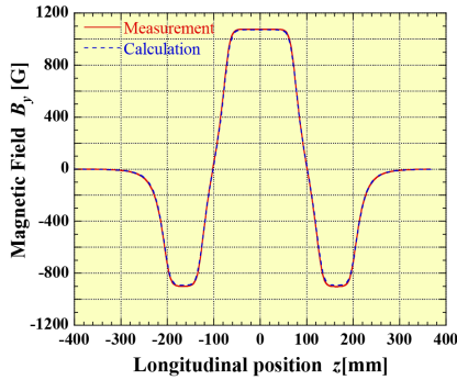
Figure 4: Measured and calculated magnetic fields of the chicane magnet along the center axis at coil currents of I_{BMIS01} = I_{BMIS03} = 6.96 A and I_{BMIS02} = 8.33 A.
