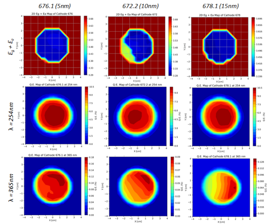
Figure 5: Maps of E_g + E_a (top row), QE at 254 nm (middle row) and 365 nm (bottom row).
