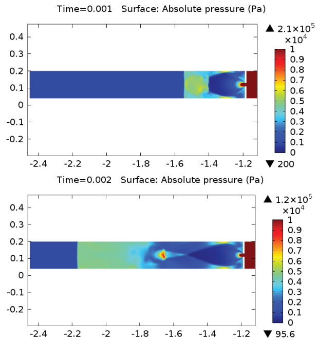
Figure 5: COMSOL simulation of pressure evolution in a tube at times 0.001s and 0.002s after opening a hole between two regions at 10^5 Pa and 10^3 Pa, with \beta=0.125 .
