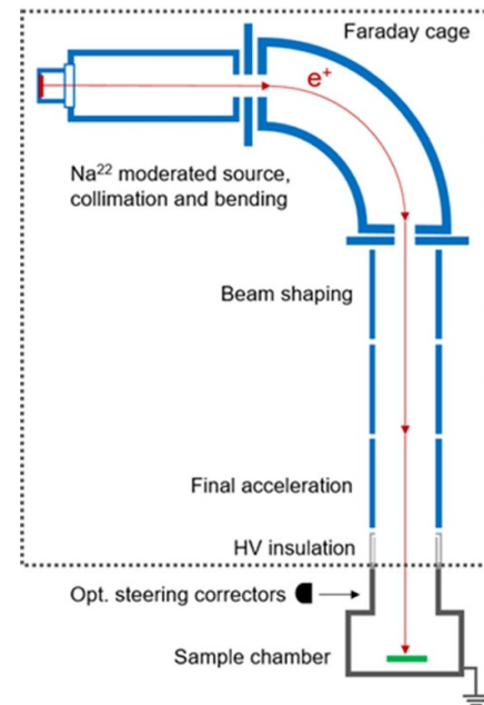
Figure 2. Schematic drawing of the electrostatic positron beamline used to characterize the detection module. Components highlighted in blue are held at a high DC negative voltage between 0 and 25 kV, whereas the sample chamber is kept at ground potential by insulating it from the acceleration stage with a ceramic vacuum section.
