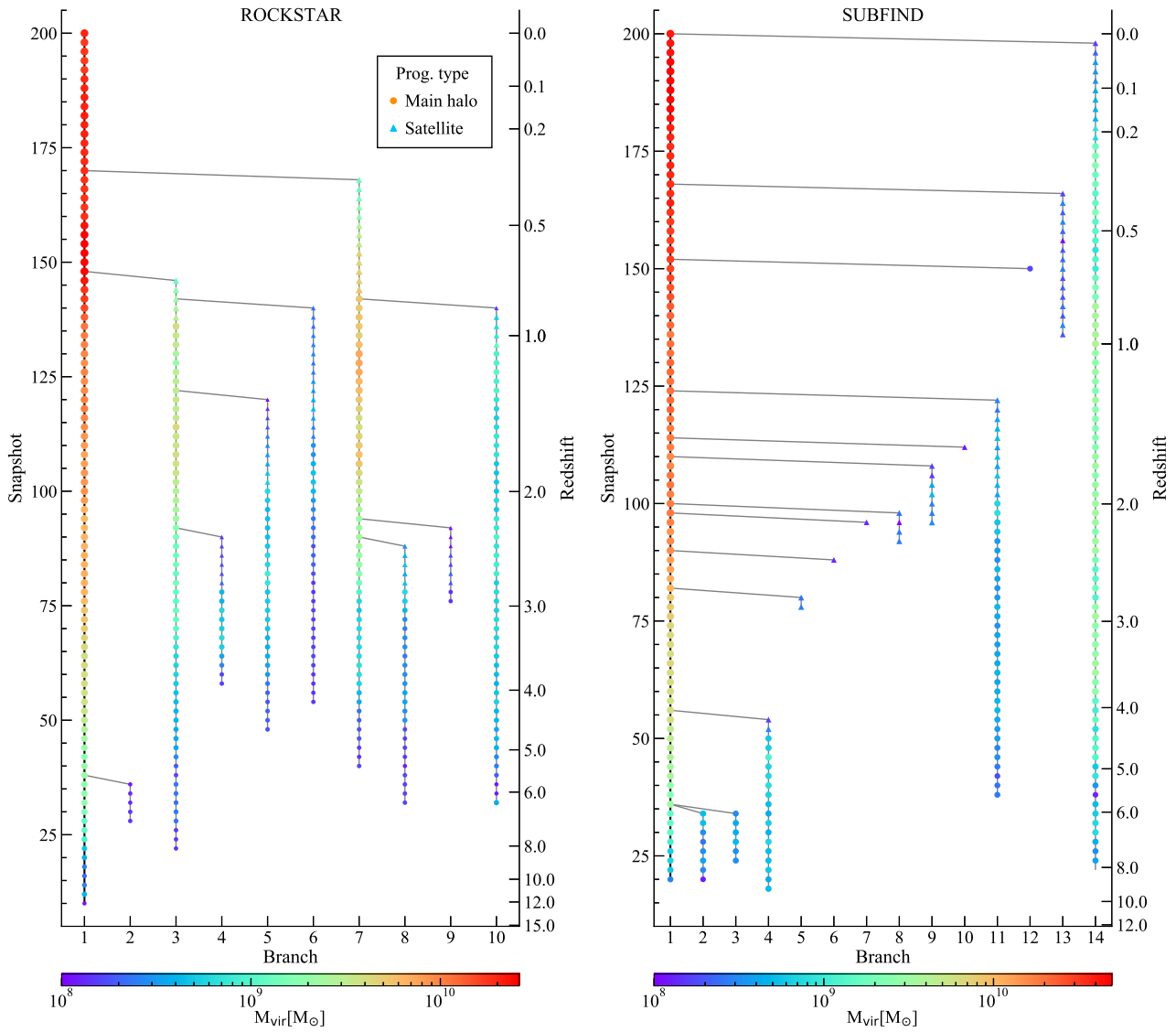
Figure B1. Additional examples of ROCKSTAR-like (left-hand panel, 10 branches) and SUBFIND-like (right-hand panel, 14 branches) ML-generated merger trees, showing the tree structure (snapshot versus branch). Progenitors that are main haloes are denoted by circles and satellites by triangles, the colour map represents the virial mass of the halo progenitors.
