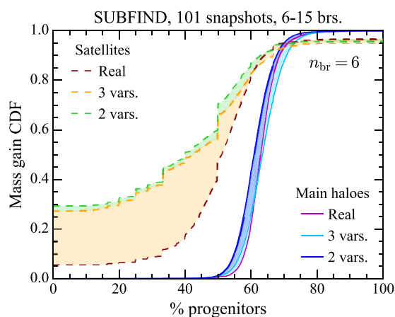
Figure 6. CDF of the mass gain for all the progenitors that are main haloes (solid) and satellites (dashed) in the SUBFIND merger tree data set with six branches, denoted ‘real’ (magenta). For comparison, we also show the CDFs for samples of trees generated with two (mass and progenitor type) and three variables. ML trees generated with a time resolution of 101 snapshots and a training data set composed of trees with number of branches in the range 6 \leq n_{\text{br}} \leq 15 . The shaded regions highlight the difference between the ‘real’ and ML CDFs.
