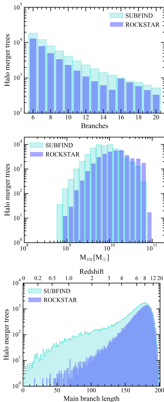
Figure 1. Histograms of the merger trees in the training data set. These are trees for main haloes at z = 0 , identified using SUBFIND – D-TREES (light blue) and ROCKSTAR – CONSISTENTTREES (blue), with number of branches in the 6 \leq n_{br} \leq 20 range (top panel). This sample corresponds to main haloes with virial masses in the 10^9 M_{\odot} \lesssim M_{vir} \lesssim 10^{11} M_{\odot} range at z = 0 (middle panel). The bottom panel shows the histogram of the length of the main branch measured in number of snapshots. The redshift axis is also shown in the top axis for reference.
