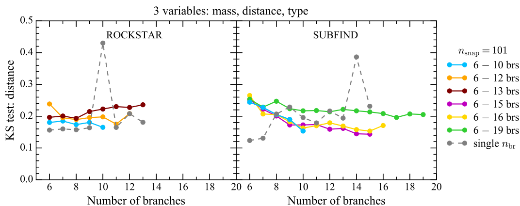
Figure 11. Snapshot averaged KS test for the distance of the progenitors to that in the main branch at the snapshot before the fusion occurs, for merger trees generated with three variables, trainings performed with either ROCKSTAR (left-hand panel) or SUBFIND (right-hand panel) merger trees.
