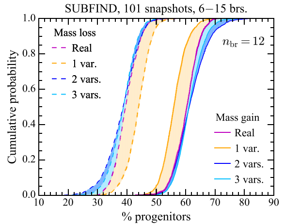
Figure 4. Cumulative distribution function (CDF) of the mass gain (solid) and loss (dashed) for all the progenitors in the SUBFIND merger tree data set with 12 branches, denoted ‘real’ (magenta). For comparison, we also show the CDFs for samples of trees generated with 1 (orange), 2 (blue), and 3 (light blue) variables, time resolution of 101 snapshots, and the GAN model trained with a data set composed of trees with 6 \leq n_{\text{br}} \leq 15 . The shaded regions depict the difference between the ‘real’ and ML CDFs.
