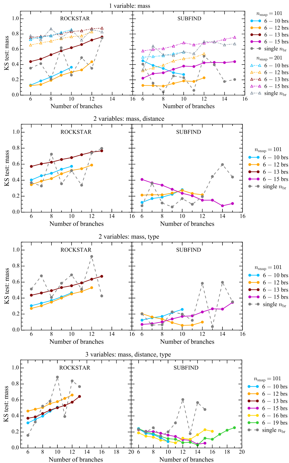
Figure 8. Kolmogorov–Smirnov (KS) test for the mass of the progenitors and the final descendant for merger trees generated with one (top panels), two (second row: mass and distance to the main branch, third row: mass and progenitor type), and three (bottom panels) input variables, GAN model trained with either ROCKSTAR (left-hand panels) or SUBFIND (right-hand panels) merger trees. Grey lines correspond to series of individual trainings (single n_{\text{br}} , one training per n_{\text{br}} ) and colourful lines to single trainings performed with trees whose number of branches varies in a range (multiple n_{\text{br}} , a single training per line).
