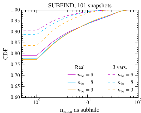
Figure 7. CDF of the number of snapshots that a progenitor is a satellite halo for the real and ML trees with n_{\text{br}} = 6, 8, \text{ and } 9 , generated with three variables (individual trainings with a time resolution of n_{\text{snap}} = 101 were performed for every n_{\text{br}} in this figure).
