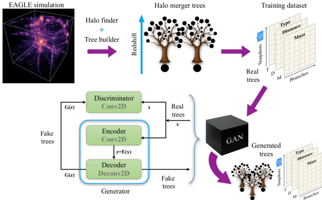
Figure 2. Halo merger tree generation process (adapted from Robles et al. 2019). Halo merger trees from the DM only EAGLE simulation of 100 cMpc constructed with either SUBFIND – D-TREES or ROCKSTAR – CONSISTENTTREES are stored in matrix format (one matrix per input variable), forming two separate data sets. Batches of these ‘real’ merger trees are the inputs of our GAN model comprised of a discriminator and a generator that consists of an encoder and a decoder, all these neural networks are made of convolutional layers (Conv2D, Deconv2D). The outputs of the GAN are batches of ‘fake’ (generated) trees in matrix format, as many matrices as input channels are obtained.
