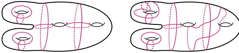
FIGURE 2 The projections of M_L(2, 2) and M_{L'}(2, 2) onto the base surface \Sigma_4 \times S^1 where L and L' are 8-component links in \Sigma_4 \times S^1
